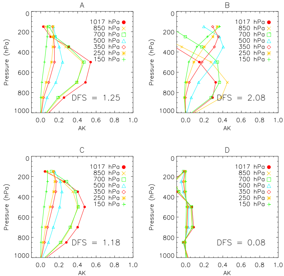
Fig. 10. Daytime and ocean averaging kernels over the Southern Africa region for 1 September 2007, for: (A) Adjusted MOPITT V3 averaging kernels converted onto the IASI pressure grid \mathbf{A}^{\text{MOP3''}} ; (B) IASI averaging kernels at pressure levels closest to the MOPITT V3 pressure levels \mathbf{A}^{\text{IASI}} ; (C) \mathbf{A}^{\text{MOP3''}} - \mathbf{A}^{\text{IASI}} ; and (D) \mathbf{A}^{\text{MOP3''}} - \mathbf{A}^{\text{MOP3''}} \mathbf{A}^{\text{IASI}} .
