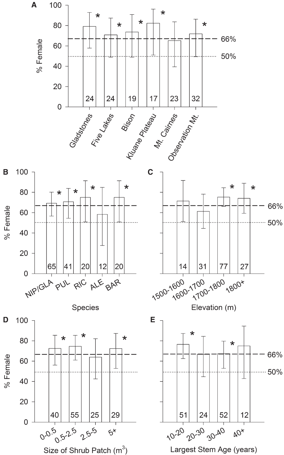
Fig. 1. Proportion of females of the species Salix niphocladalglauca (NIP/GLA), S. pulchra (PUL), S. richardsonii (RIC), S. alaxensis (ALE), and S. barrattiana (BAR) by (A) mountain valley, (B) species, (C) elevation of sampling, (D) patch size class, and (E) stem age. Species are pooled in plots A, C, D, and E. Error bars indicate binomial confidence intervals and the number in each bar indicates sample size. Asterisks indicate sex ratios that differ significantly from a 1♀:1♂ sex ratio (dotted line, \chi^2 , P < 0.05 ); no sex ratios differ significantly from a 2♀:1♂ sex ratio (dashed line, \chi^2 , P < 0.05 ).
