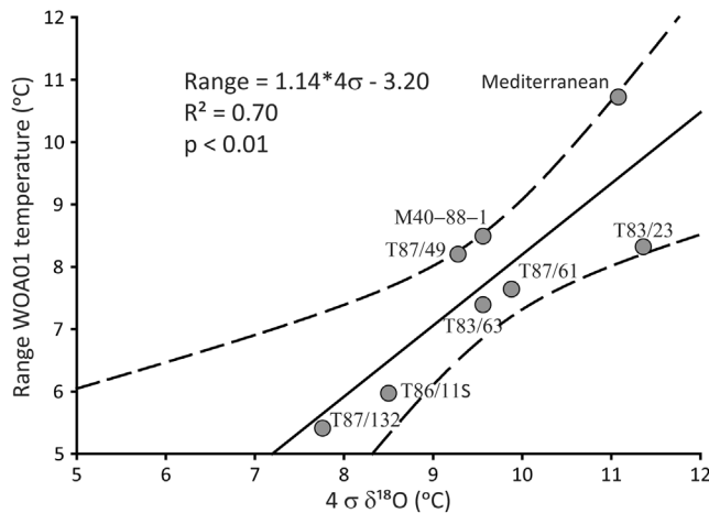
Figure 7. Four standard deviations of \delta^{18}\text{O} -derived temperatures versus the range (max-min) in WOA01 temperature for each sample location with 95% confidence limit of the standard deviation being less than 2°C. The Mediterranean data point is obtained by combining all measured \delta^{18}\text{O} data from the Mediterranean box cores, including stations with too large confidence limits for the standard deviations, and comparing them to the combined database temperatures of those same box cores. This results in all other data plotted in Figure 7 also being included in the Mediterranean data point, potentially biasing the independency of this point. The correlation coefficient is significant at the 99% level ( p < 0.01 ). The dotted lines represent the 95% confidence limits of the regression line but do not include the 95% confidence interval as calculated for each site in Table 2.
