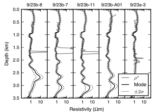
Figure 10. Well logs (gray) and the mode (black) and \pm 2\sigma (dashed) of the resistivity predictions calculated using the seismic velocities. Well 9/23b-8 (leftmost) is the calibration well. The same transform applied to four wells on Harding Central shows a good match: Most well measurements lie within \pm 2\sigma . High resistive, hydrocarbon-bearing formations are not predicted because we assume brine-filled pores. Shallow, sandy sections are also poorly resolved, except for the Grid sandstones, which we explicitly incorporated into our model.
