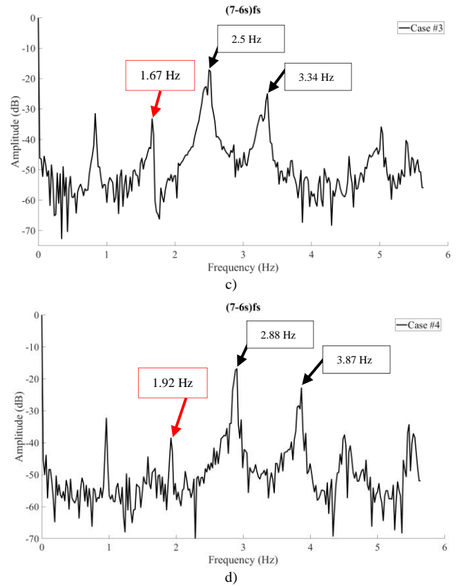
Fig. 11. FFT spectra of each S(t, f_{7,1}) for the spectral component (7-6s)fs of: a) Case #1 b) Case #2 c) Case #3 d) Case #4. \Delta f = 0.5 Hz.
