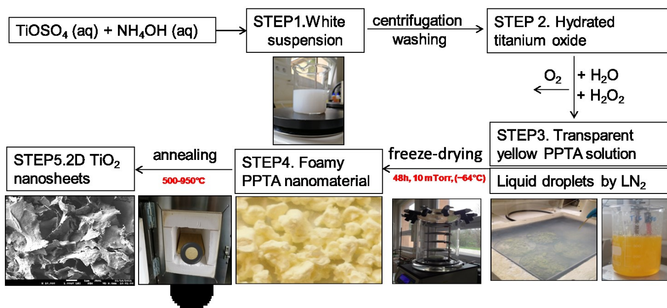
Figure 1. Schematic of the preparation procedure of PPTA precursor and the 2D \text{TiO}_2 nanosheets.
