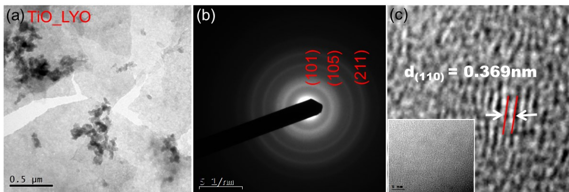
Figure 4. (a) TEM image of pristine sample TiO_LYO (b) SAED pattern of TiO_LYO indexed to the orthorhombic hydrogen titanium oxide hydride H_4Ti_2O_6 \cdot H_2O (c) HRTEM image of TiO_LYO with interlayer distance d confirms H_4Ti_2O_6 \cdot H_2O structure.
