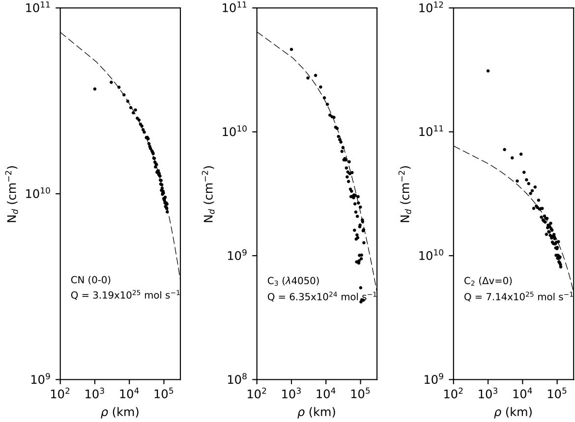
Figure 6. The extracted spatial profiles for comet C/2014 S2. The production rates determined using the C12 scale lengths are given for each emission feature, and the corresponding Haser profile for that production rate is plotted as a dashed line. The OH and NH scale lengths are the same as those in AH95 and the plots for these features are not repeated here.
