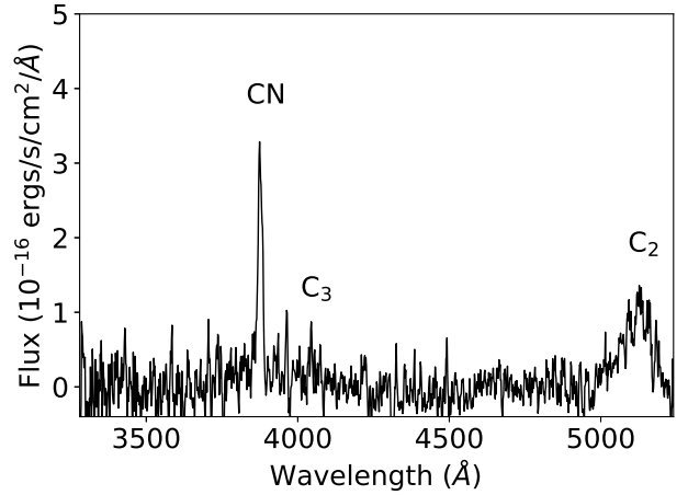
Figure 3. Extracted dust-subtracted blue arm spectrum of comet 116P/Wild 4. The molecular gas emission bands are labelled.
