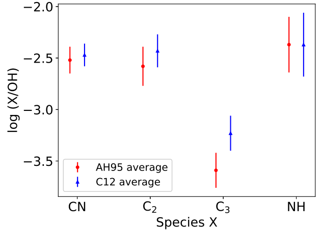
Figure 7. Comparison plot of average log ratios of each species X to OH.
