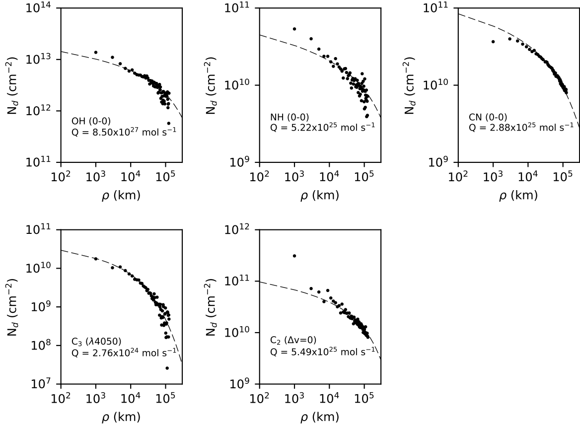
Figure 5. The extracted spatial profiles for comet C/2014 S2. The gas emission for this comet extends over the length of the slit. The production rates determined using the AH95 scale lengths are given for each emission feature, and the corresponding Haser profile for that production rate is plotted as a dashed line.
