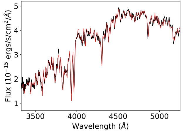
Figure 4. Extracted spectrum of cometary fragment P/2016 BA14. The fitted solar spectrum is plotted in red.
