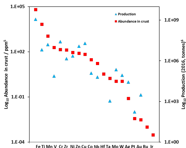
Fig. 4 Abundance of selected elements for use in the formation of PCs.
