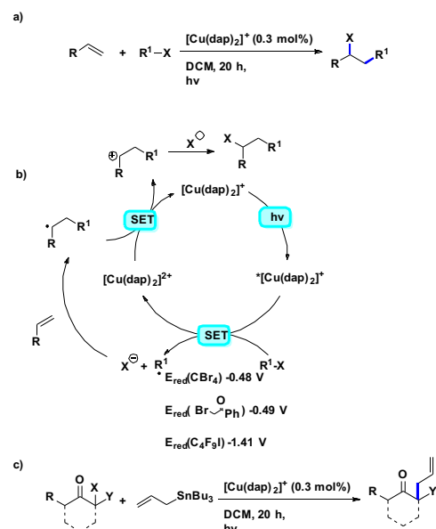
Fig. 13 a) ATRA reactions of halides and olefins; b) proposed mechanism by Reiser et al. ; c) Visible-light-induced [Cu(dap) 2 ]Cl catalysed allylation of \alpha -halocarbonyl compounds
