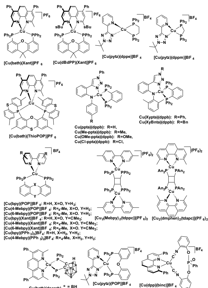
Fig. 6 [\text{Cu}(\text{N}^{\wedge}\text{N})(\text{P}^{\wedge}\text{P})]^+ and [\text{Cu}(\text{N}^{\wedge}\text{N})(\text{P}^{\wedge}\text{P})] type complexes.
