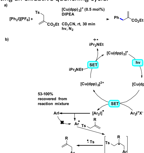
Fig. 21 Reductive arylation of allyl-tosylates by Ollivier et al. ; the photoreduction of aryl iodides was discussed by Sauvage et al. 87
