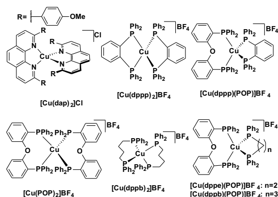
Fig. 7 [\text{Cu}(\text{N}^{\wedge}\text{N})_2]^+ and [\text{Cu}(\text{P}^{\wedge}\text{P})_2]^+ complexes.
