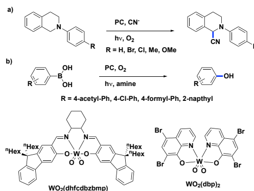
Fig. 38 a) Oxidative cyanation of tertiary amines photocatalyzed by WO 2 (dhfcdzbzmp) and WO 2 (dbp) 2 (where R=C 6 H 5 instead of Br); b) Oxidative hydroxylation of aryl boronic acids photocatalyzed by WO 2 (R-dbp) 2 where R=C 6 H 5
