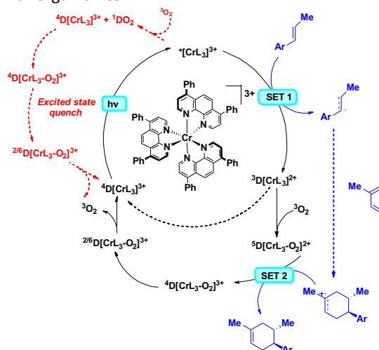
Fig. 43 Proposed mechanism of photocatalysis using [\text{Cr}(\text{Ph}_2\text{phen})_3]^{3+} .
