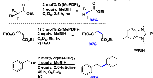
Fig. 39 Reactions tested using Zr(MePDP) 2 as photocatalyst.
