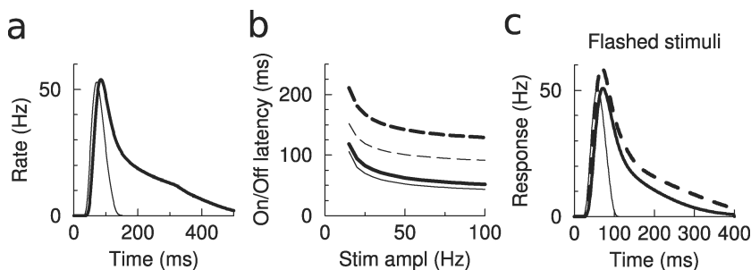
Figure 7: The effect of a slow NMDA-like current on the model. In each panel, the network with NMDA is shown in thick curves; the model without NMDA is shown in thin curves for comparison. (a) The response in the fifth layer to a 300 ms step stimulus. With NMDA, a sustained response results similar to what is seen in some recorded cells. (b) The onset latency (solid curve) and offset latency (dashed curve) as a function of stimulus. The onset latency is only slightly changed with NMDA, but the offset latency is extended considerably. (c) The response in the fifth layer to flashed stimuli as used in Figure 4. The NMDA component again lengthens the response, but the response remains insensitive to precise stimulus duration. Solid curve: response to brief stimuli; dashed curve: response to long stimuli.
