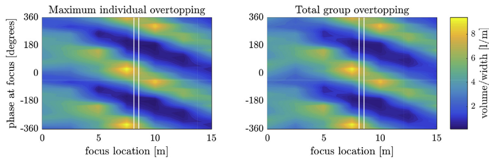
Fig. 12. Maximum overtopping volumes generated by incident focused wave groups of amplitude 0.114 m for varying focus location and phase at focus.
