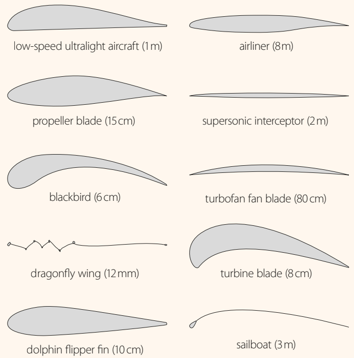
3 Examples of aerofoil profiles in Nature and in various vehicles.
