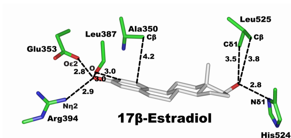
Figure 7. Structure of ER \alpha with 17 \beta -estradiol [34, 117].
