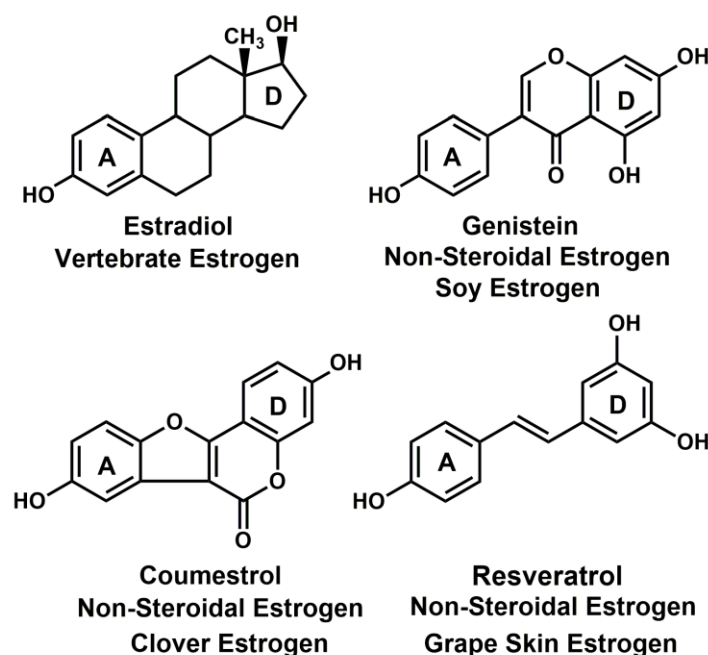
Figure 5. Chemicals from plants that act as estrogens.
