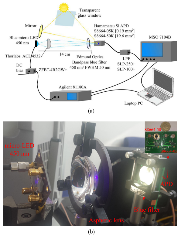
Fig. 7. The experimental set-up. (a) Schematic set-up of the experiment showing the optical system, arbitrary waveform function generator, oscilloscope, electrical and optical filters and Bias-T. (b) Photograph of the optical system showing the micro-LED, optical lenses system and the used APDs. In the top right corner (left): large APD s8664-50k; (right): small APD S8664-05k.
