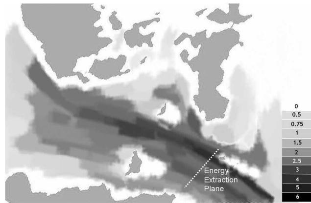
Fig. 7 Location of energy flux plane
