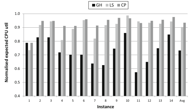
Fig. 4 Expected CPU utilisation for greedy heuristic (GH), local search (LS), and constraint programming (CP). Values are normalised to the corresponding total CPU capacity (= 1). Server capacity = 400
