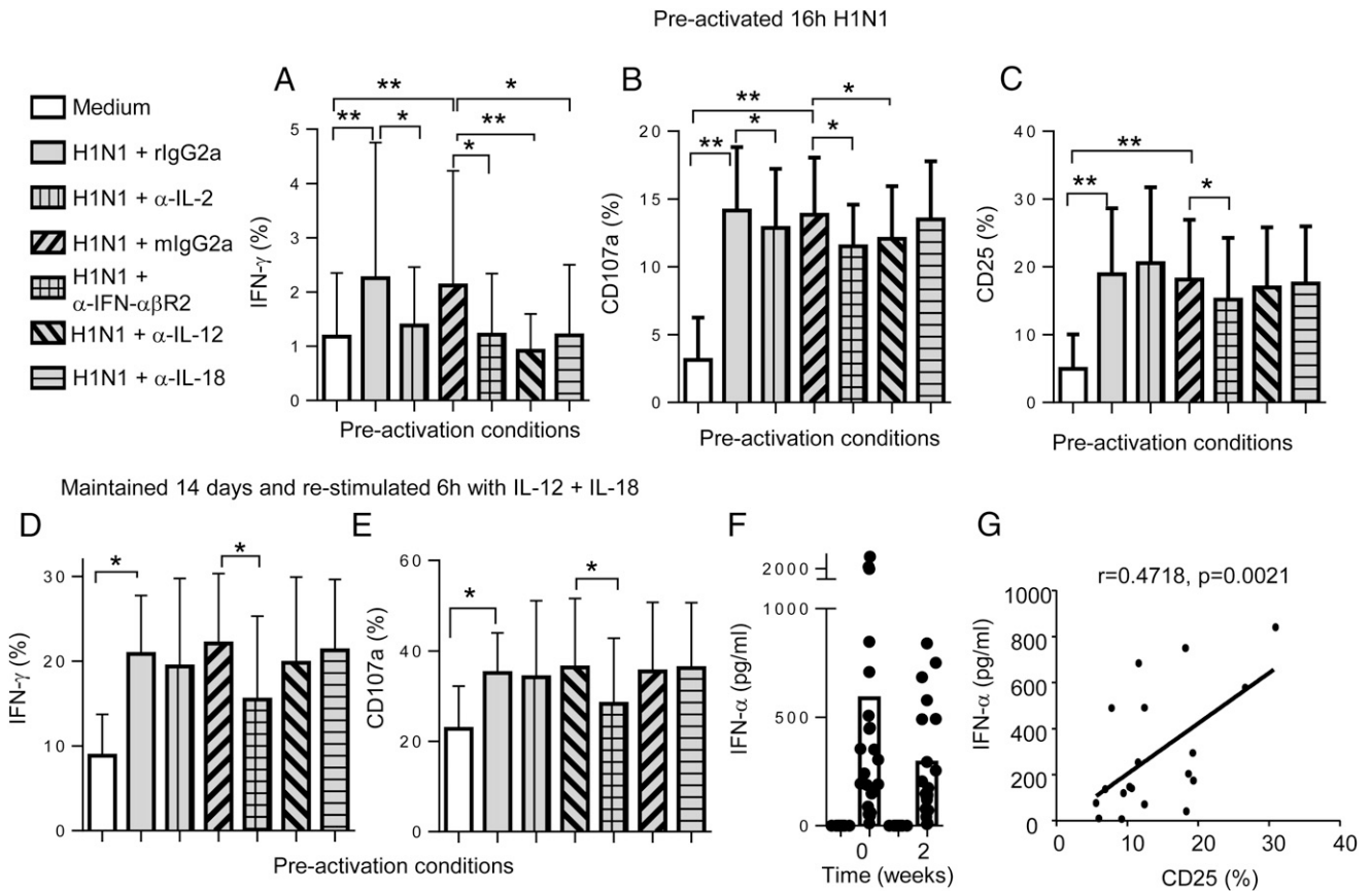
FIGURE 6. IFN- \alpha 2R2 blockade abrogates in vitro preactivation of NK cells by influenza virus (A–E). PBMCs from eight individuals were preactivated with H1N1 in the presence of neutralizing anti-IL-2, anti-IL-12, anti-IL-18, or blocking anti-IFN- \alpha 2R2 Ab or rat or mouse isotype control reagents, as indicated. The frequencies of NK cells expressing IFN- \gamma (A and D), CD107a (B and E), or CD25 (C) after 6-h restimulation with HCC (IL-12 5 ng/ml plus IL-18 50 ng/ml) were measured directly (A–C) or after maintenance in IL-15 replete medium for 14 d (D and E). (F) IFN- \alpha concentrations in culture supernatants of H1N1-stimulated PBMCs from 32 individuals (17 HCMV ^{-} , 15 HCMV ^{+} ) before (0) and 2 wk after vaccination. (G) Correlation between H1N1-induced IFN- \alpha concentration and H1N1-induced CD25 expression 2 wk postvaccination. Statistical comparisons between NK cells with and without preactivation or between different neutralizing/blocking conditions were made by Mann-Whitney U test. * p < 0.05 , ** p < 0.01 .
