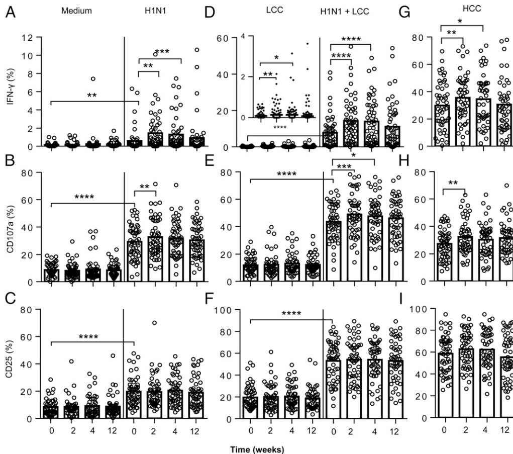
FIGURE 2. NK cell responses to influenza viruses are enhanced after influenza vaccination. PBMC were collected from 52 study subjects prior to (week 0) or after vaccination (weeks 2, 4, and 12) and cultured in vitro in culture medium alone, with vaccine strain influenza H1N1 ( A–C ) or with LCC (IL-12 12.5 pg/ml plus IL-18 10 ng/ml) alone or combined with H1N1 ( D–F ). Responses to HCC (IL-12 5 ng/ml + IL-18 50 ng/ml) were also determined before and after vaccination ( G–I ). Expression of IFN- \gamma ( A, D, and G ), CD107a ( B, E, and H ), and CD25 ( C, F, and I ) were analyzed within the total NK cell population. Paired statistical comparisons of NK cell responses before and after vaccination and between virus or cytokine responses and untreated cultures (medium) were performed using Wilcoxon signed-rank test. * p < 0.05 , ** p < 0.01 , *** p < 0.001 , **** p < 0.0001 .
