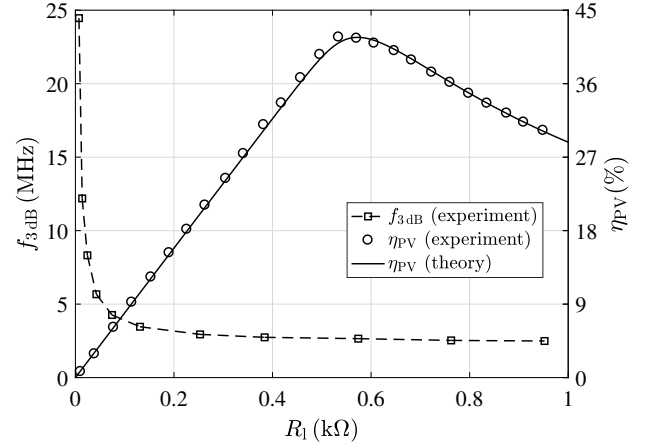
Fig. 3. Bandwidth of 3 dB and power efficiency of the PV cell as a function of load resistance.
