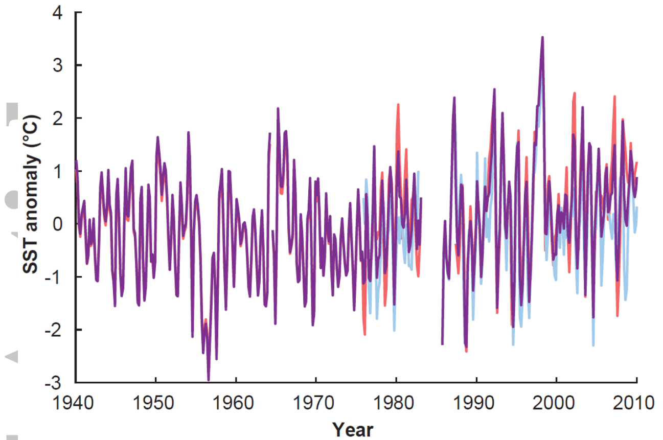
Figure 2. Bimonthly reconstructed SST anomalies (relative to mean bimonthly values) for the Wolf composite record ( \text{Sr}/\text{Ca} = 10.66 - 0.057 \cdot \text{SST} ), showing the composite (purple), GW10-3 (blue), and GW10-10 (light red). The 1982-83 El Niño caused a growth hiatus from 1983-1985.
