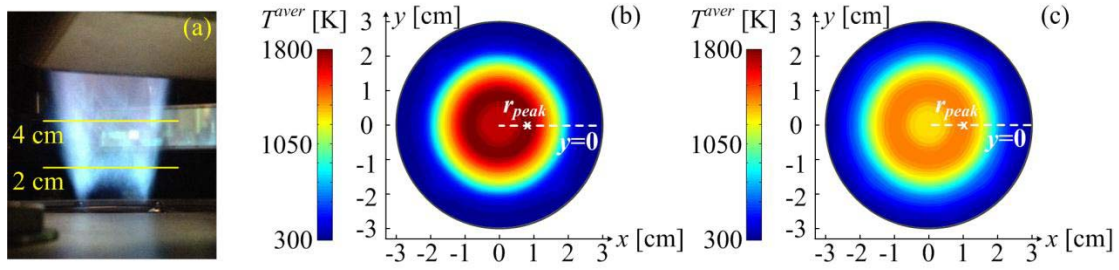
Fig. 8. (a) Photograph and averaged tomographic images of temperature over the cross section of interest in the swirling flame at (b) z = 2 cm and (c) z = 4 cm when the flows of methane and air are 8 and 371 L/min, respectively.
