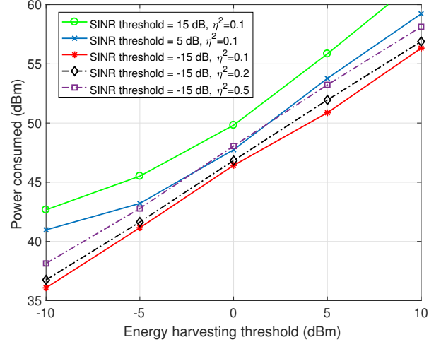
Fig. 6. Power consumption of imperfect FD MIMO interference channel for different SINR thresholds and error bounds.
