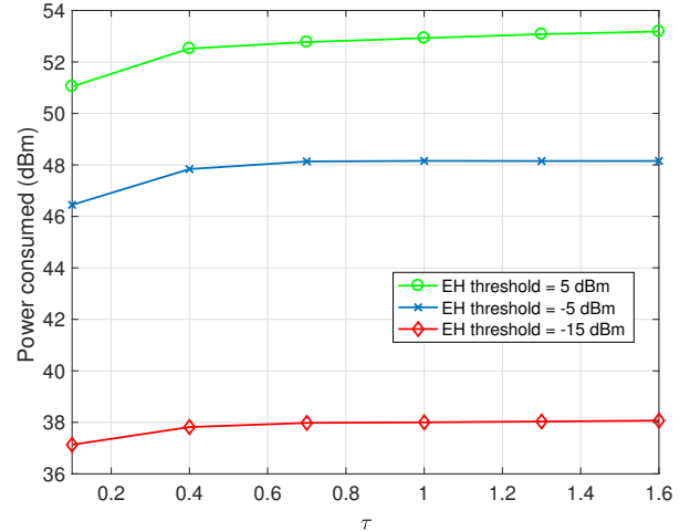
Fig. 7. Power consumption of imperfect FD MIMO interference channel for different values of \tau and EH thresholds.
