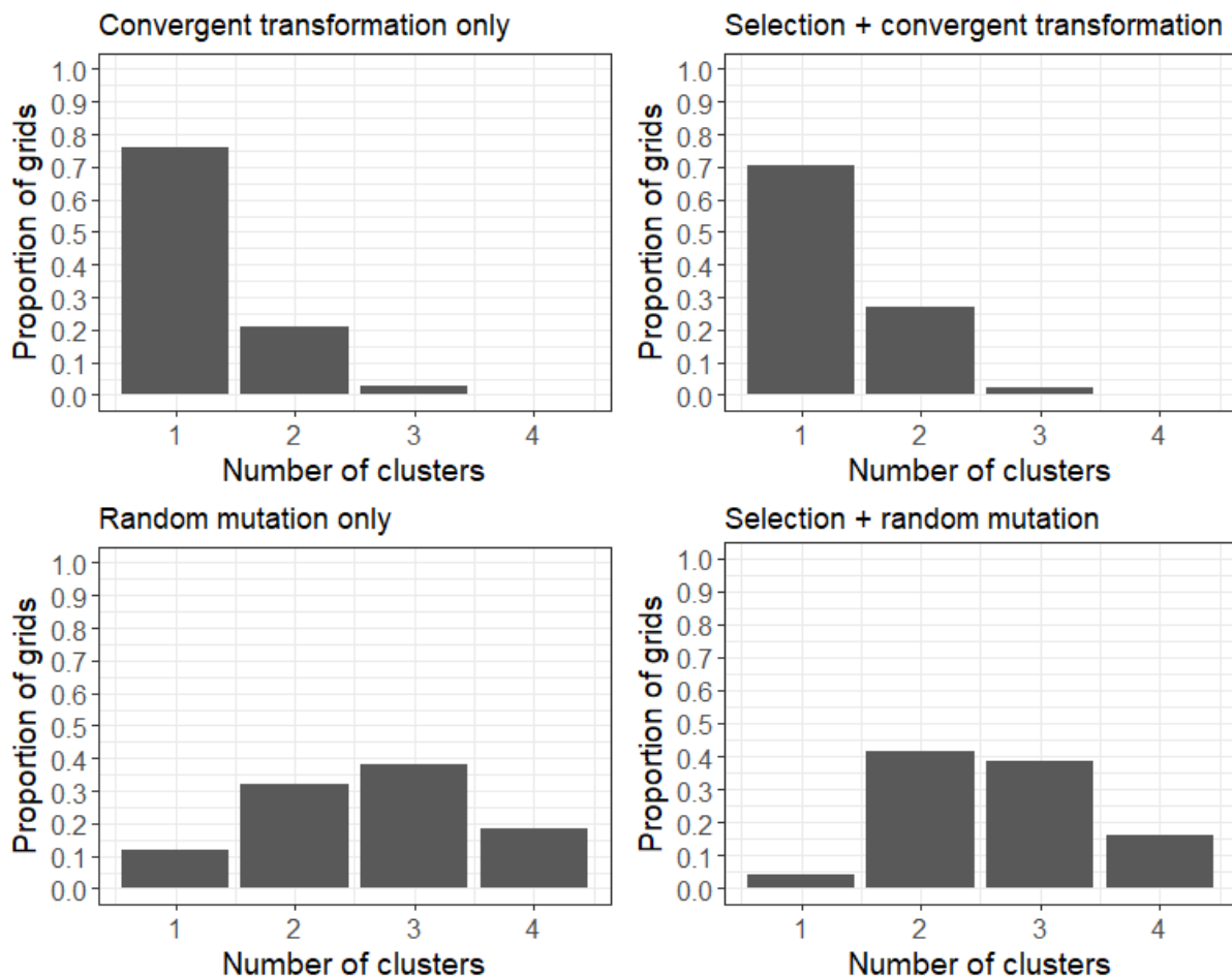
Figure 9: Proportion of grids with different number of clusters inferred from simulations with convergent transformations or random mutations, and with or without selection. The selection pressure is set at 10 grids and the grids are selected for maximal distance.
