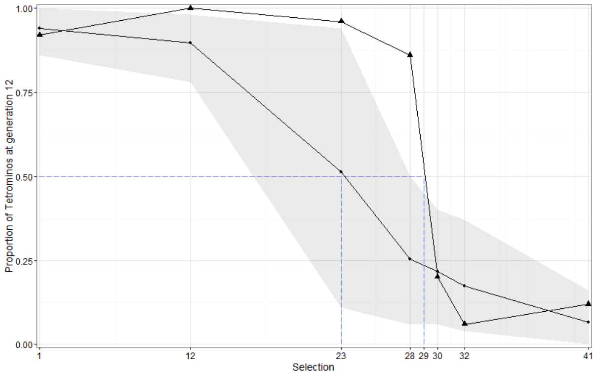
Figure 7: Observed and simulated proportion of tetromino at generation 12. Dots represent the average proportion of tetromino obtained through simulations (the grey area represents the 95% confidence interval of the proportion) and triangles the results obtained during the experiment. The dotted blue lines show the selection values at PE.
