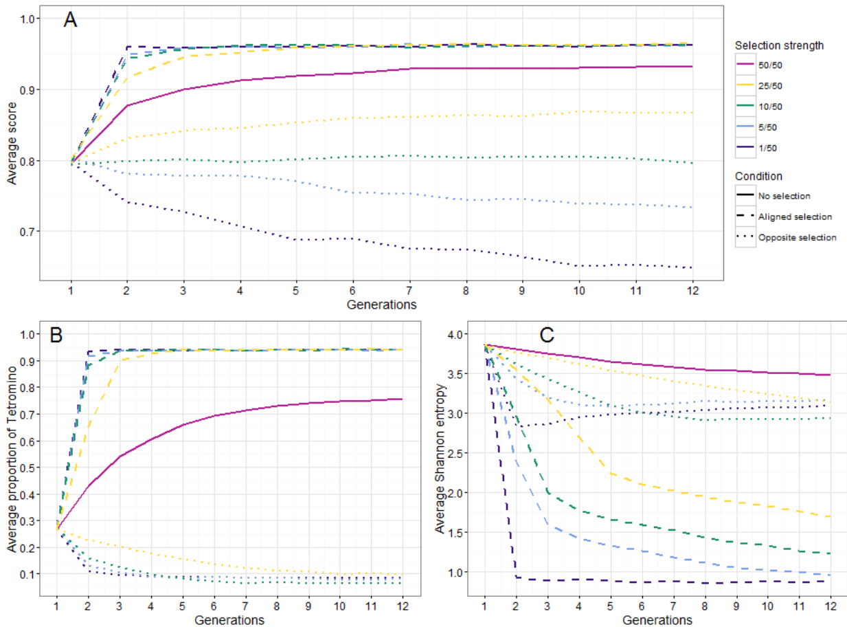
Figure 3: Effect of selection on cultural evolution. Evolution of the score (A), number of tetrominoes (B) and Shannon entropy (C) in the absence of selection (solid line), with aligned selection (dashed lines) and with opposite selection (dotted lines). The colours represent variations in selection pressure, from 50 grids selected in the set of 50 (i.e. no selection) to 1 grid selected in the set (i.e. maximal selection).
