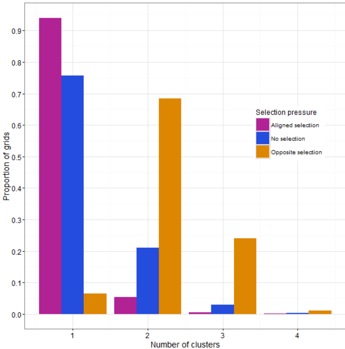
Figure 5: Number of clusters at generation 12 in three conditions: no selection, aligned selection and opposite selection. Selection pressure is set at 10 grids.
