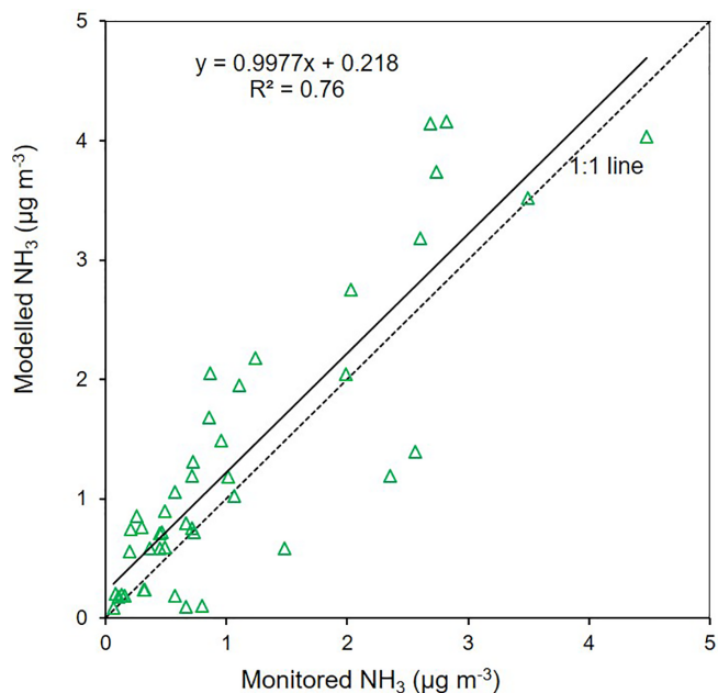
Figure 6. Comparison of 2012 annual mean concentrations of \text{NH}_3 from output of the FRAME atmospheric model with measurements from the UK National Ammonia Monitoring Network (NAMN) for a subset of sites classified as located in semi-natural or forest locations.
