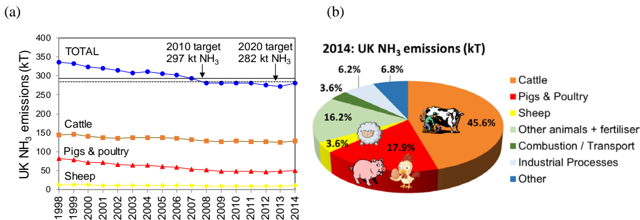
Figure 10. (a) Trends between 1998 and 2014 in the UK National Atmospheric Emission Inventory (NAEI) for total UK \text{NH}_3 emissions and selected sub-sources: cattle, pigs & poultry and sheep. The 2010 \text{NH}_3 national emissions ceiling target of 297 kt (Gothenburg protocol and NECD) and the 2020 target of 282 kt (revised Gothenburg protocol) are also shown for comparison. (b) UK \text{NH}_3 emission sources in 2014. Data from http://naei.defra.gov.uk/ and Misselbrook et al. (2015).
