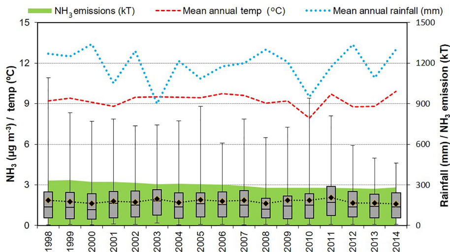
Figure 11. Changes in annual mean atmospheric \text{NH}_3 concentrations averaged over all sites in the National Ammonia Monitoring Network (NAMN) operational between 1998 and 2014 (59 sites). The diamonds show the mean \text{NH}_3 concentration, with the grey box indicating the median and interquartile range, while the error bars show the range (minimum and maximum) of measured mean concentrations. Annual mean UK meteorological data (source http://www.metoffice.gov.uk/ ) are also plotted for comparison over the same period. 2010 was an unusual year, characterized by a considerably lower than average mean annual temperature of 7.9^\circ\text{C} due to an exceptionally cold winter, with December 2010 recorded as the coldest for over 100 years (cf. mean = 9.2^\circ\text{C} for 1998 to 2014) and lower than average rainfall of 950 mm (cf. mean = 1190 mm for 1998 to 2014).
