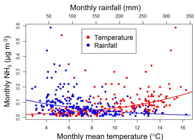
Figure 9. Relationships between measured monthly-mean \text{NH}_3 concentrations from the UK National Ammonia Monitoring Network (NAMN) and mean monthly temperature and rainfall at Inverpollly (UKA00457). \text{NH}_3 was negatively correlated with rainfall (blue line: \text{Log}(\text{NH}_3) = -0.0059 \times \text{Log}(\text{rain}) - 2.1612 , R^2 = 0.19 , n = 231 , p < 0.05 ) and positively correlated with temperature (red line: \text{Log}(\text{NH}_3) = 0.1482 \text{Log}(\text{temp}) - 4.2708 , R^2 = 0.33 , n = 231 , p < 0.05 ). Rain and temperature data are from the nearby Aultbea meteorological station (ID no. 52; Met Office, 2016).
