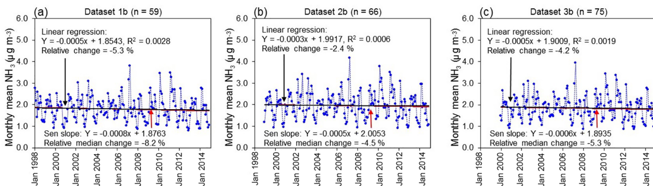
Figure 13. Time series trend analysis by non-parametric Mann–Kendall Sen slope vs. parametric linear regression on monthly mean \text{NH}_3 concentrations from the UK National Ammonia Monitoring Network (NAMN) for (a) dataset 1b (1998–2014, n = 59 ), (b) dataset 2b (1999–2014, n = 66 ) and (c) dataset 3b (2000–2014, n = 75 ). Individual data points are monthly mean \text{NH}_3 concentrations.
