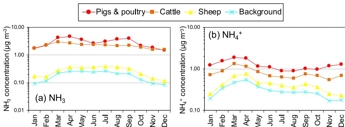
Figure 7. Seasonal trends in (a) \text{NH}_3 (mean monthly data for 1998–2014) and (b) \text{NH}_4^+ (mean monthly data for 1999–2014) concentrations of sites in the UK National Ammonia Monitoring Network (NAMN) classified according to four key emission source categories: cattle, sheep, pigs & poultry and background (based on 2005 dominant emission source classification). The concentrations are plotted on a log scale for better visualization of the low-concentration background and sheep profiles.
