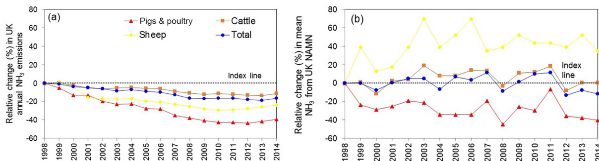
Figure 16. (a) Relative trends between 1998 and 2014 in \text{NH}_3 emissions from the UK National Atmospheric Emission Inventory (NAEI) for total emissions (all \text{NH}_3 sources) and emissions from cattle, pigs & poultry, and sheep separately (data from http://naei.defra.gov.uk/ and Misselbrook et al., 2015). (b) Relative trends between 1998 and 2014 in measured annual mean \text{NH}_3 concentrations ( \mu\text{g NH}_3 \text{ m}^{-3} ) for all UK National Ammonia Monitoring Network (NAMN) sites, and for grouped sites classified as dominated by cattle, pigs & poultry, and sheep. Both figures are plotted with the same scale to allow direct comparison of the relative magnitudes in trends.
