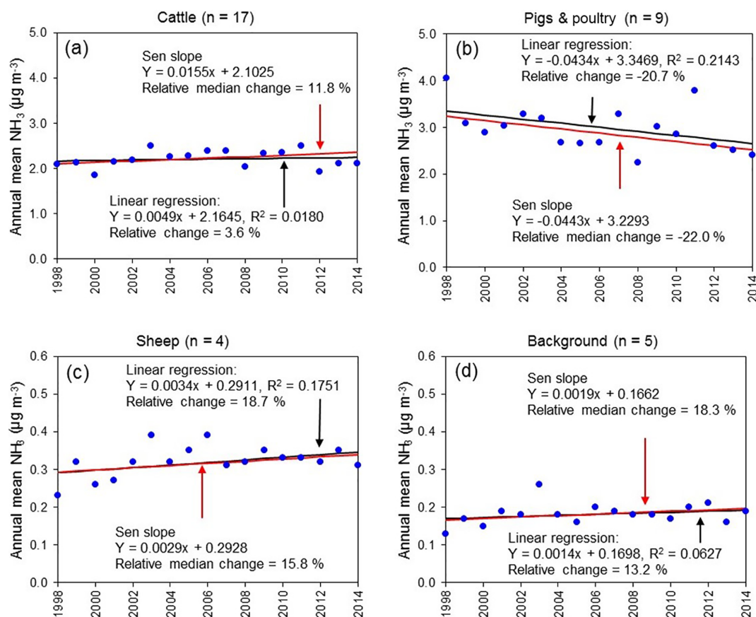
Figure 14. Time series trend analysis by non-parametric Mann–Kendall Sen slope vs. parametric linear regression on annually averaged \text{NH}_3 concentrations from the UK National Ammonia Monitoring Network (NAMN) for sites in 5 km grid squares classed as dominated by (a) cattle (>45 % of total \text{NH}_3 emissions from this category in a grid square); (b) pigs & poultry (>45 % of total \text{NH}_3 emissions from this category in a grid square); (c) sheep (>45 % of total \text{NH}_3 emissions from sheep in a grid square); (d) NAMN sites in grid squares classed as background (defined as grid squares with average \text{NH}_3 emissions < 1 \text{ kg N ha}^{-1} \text{ yr}^{-1} ). Individual data points are annually averaged \text{NH}_3 concentrations.
