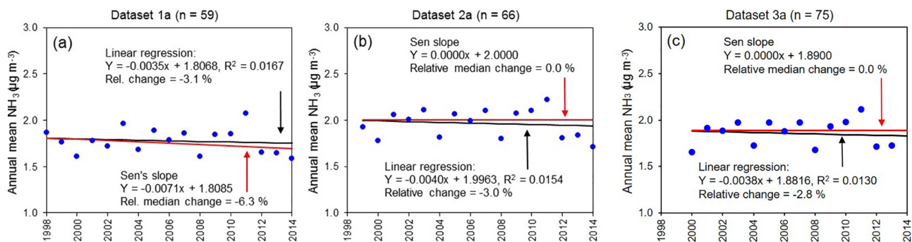
Figure 12. Time series trend analysis by non-parametric Mann–Kendall Sen slope vs. parametric linear regression on annually averaged \text{NH}_3 concentrations from the UK National Ammonia Monitoring Network (NAMN) for (a) dataset 1a (1998 to 2014, n = 59 ), (b) dataset 2a (1999 to 2014, n = 66 ) and (c) dataset 3a (2000 to 2014, n = 75 ). Individual data points are annually averaged \text{NH}_3 concentrations.
