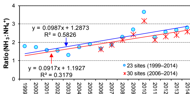
Figure 17. Long-term trends in ratio of \text{NH}_3 : \text{NH}_4^+ , indicating an increase in this ratio with time. The comparisons shown is for datasets (i) 23 sites with complete \text{NH}_4^+ time series from 1999 to 2014, and (ii) 30 sites with complete \text{NH}_4^+ time series from 2006 to 2014.
