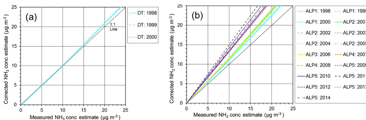
Figure 2. Comparison of annual empirical calibration curves for the passive samplers against the reference estimates from DELTA sampling at more than 9 sites in the UK National Ammonia Monitoring Network (NAMN). (a) DT, diffusion tubes. (b) ALP, ALPHA samplers; ALP1 is prototype 1 (1998–2000), ALP2 (2001–2005) and ALP3–ALP5 were manufactured from injection moulds 1 and 2, respectively. ALP4 and ALP5 have new inlet PTFE membrane (Swiftlab 07-OPM-027, 305 µm, regular polypropylene grid support material) that replaced the previous TE38 PTFE membrane (265 µm, randomly arranged polypropylene support material). ALP5: at new laboratory with analysis on FloRRia (previously on AMFIA).
