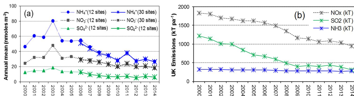
Figure 18. (a) Long-term trends in particulate \text{NH}_4^+ from the UK National Ammonia Monitoring Network (NAMN) compared with particulate \text{NO}_3^- and \text{SO}_4^{2-} concentrations from the UK Acid Gases and Aerosols Monitoring Network (AGANet; Conolly et al., 2016) measured at the same time. Each data point represents the averaged monthly measurements from all AGANet sites (increased from 12 to 30 sites since January 2006) and also the original 12 AGANet sites in the network (1999 data were excluded as measurements started in September 1999). (b) Trends in total UK emissions of \text{NH}_3 , \text{NO}_x and \text{SO}_2 over the same period (2000–2014). Data from the National Atmospheric Emission Inventory (NAEI, http://naei.defra.gov.uk/ ).
