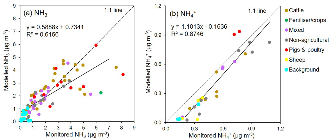
Figure 5. Comparison of 2012 annual mean concentrations of (a) \text{NH}_3 and (b) \text{NH}_4^+ modelled using the FRAME atmospheric model with 2012 measurements from the UK National Ammonia Monitoring Network (NAMN) for all sites according to dominant emission source classification.
