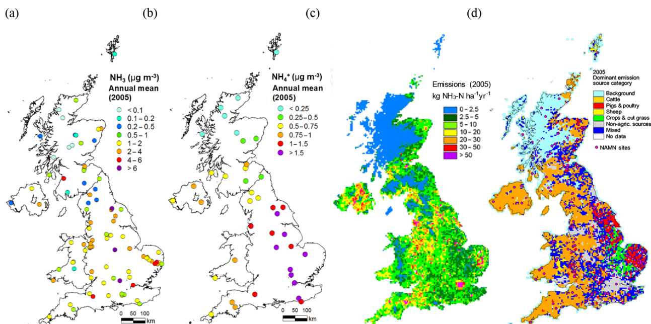
Figure 4. Measured annual mean concentrations from the UK National Ammonia Monitoring Network (NAMN) for 2005 for (a) \text{NH}_3 and (b) particulate \text{NH}_4^+ , and maps at 5 km by 5 km grid resolution for 2005 of (c) the estimated annual \text{NH}_3 emissions (Dragosits et al., 2005) and (d) the dominant \text{NH}_3 emission source category (based on Hellsten et al., 2008), indicating the relationships between measured air concentrations and spatial variability in \text{NH}_3 emission sources. The measurements show a broad pattern of small air concentrations across NW Scotland. Conversely, the largest concentrations occur in areas with intensive cattle, pig and poultry farming with high \text{NH}_3 emissions – e.g. East Anglia in SE England.
