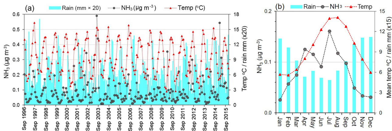
Figure 8. (a) Long-term trends in measured monthly-mean \text{NH}_3 concentrations at the remote background Inverpollly site in NW Scotland (UKA00457), demonstrating strong intra- and inter-annual variability, from the UK National Ammonia Monitoring Network (NAMN). Also plotted for comparison are monthly rainfall and temperature data from the nearby Aultbea meteorological station (ID no. 52; Met Office, 2016). (b) Comparison of seasonal trends in \text{NH}_3 concentrations with temperature and rainfall at Inverpollly. Data shown are averaged over the period 1996–2015. Peak concentrations of \text{NH}_3 can be seen to coincide with summer maxima in the temperature profile, while the lowest concentrations occur in winter when the temperature is lowest and also when rainfall is generally highest.
