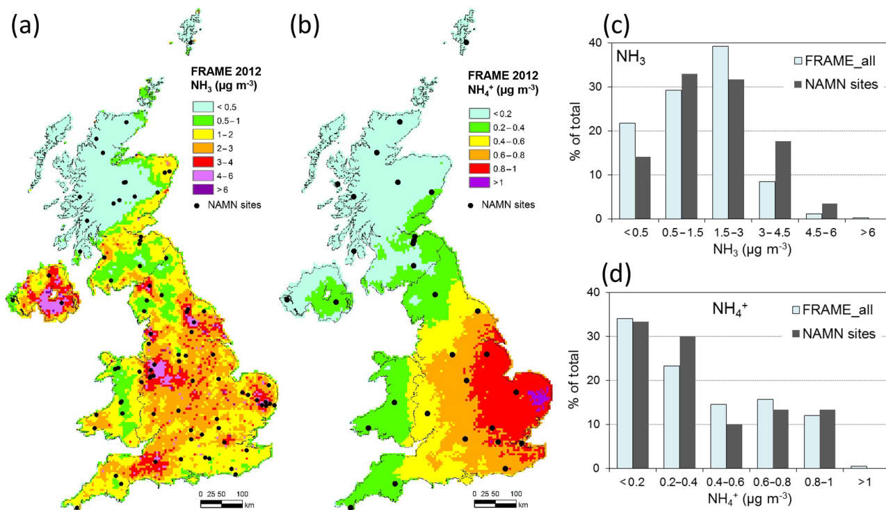
Figure 1. Maps of modelled annual mean concentrations of (a) NH 3 and (b) NH 4 + at 5 km × 5 km grid resolution from the FRAME atmospheric transport model using 2012 UK emissions data, based on Dore et al. (2008), overlaid with the National Ammonia Monitoring Network (NAMN) measurement sites, and frequency distributions of the modelled concentrations of (c) NH 3 and (d) NH 4 + for the FRAME 5 km grid squares containing a NAMN site (85 and 30 sites, respectively, in 2012) and for all model grid squares over the UK.
