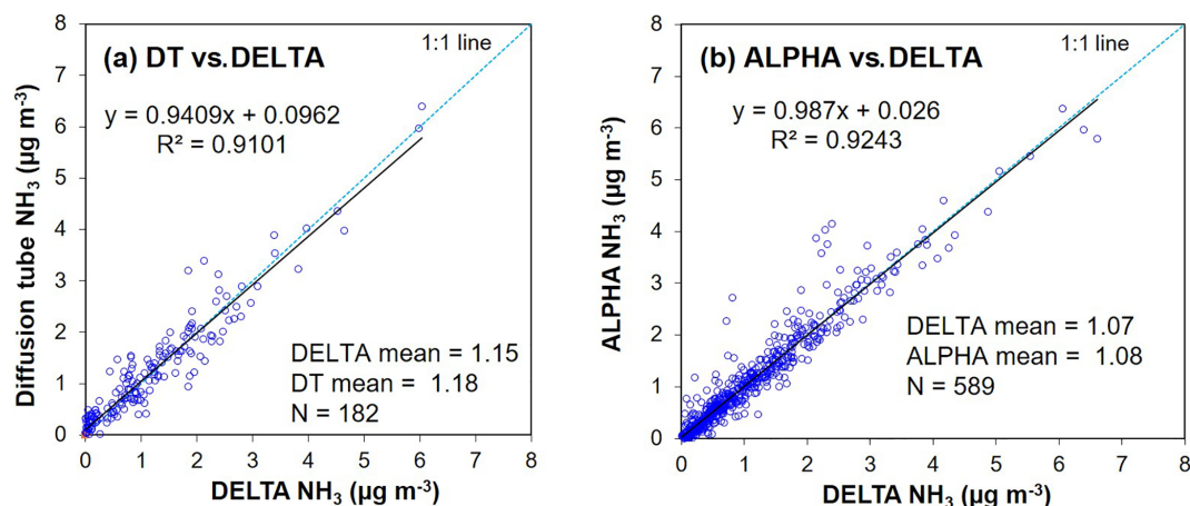
Figure 3. Regression of passive samplers vs. DELTA measurements at more than 9 sites in the UK National Ammonia Monitoring Network (NAMN), showing results for (a) diffusion tubes (DT), used during the early years of the network (1998–2000), and (b) for ALPHA samplers (results shown are for 2009–2014 where all analyses were carried out at a new laboratory). All passive data shown are the monthly measured concentrations for each site using the calibrated data for the respective passive methods.
