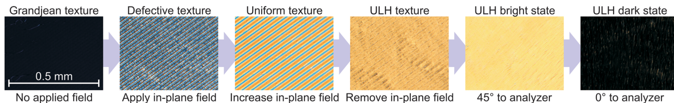
FIG. 3. (Color online) Schematic diagram of the uniform lying helix texture induction process using interdigitated electrodes. Application of low frequency, in-plane ( V_2, V_3 ) fields induce defects, which relax into the ULH alignment after the removal of the field. Flexoelectro-optic switching is achieved by applying a voltage across the connected in-plane electrodes ( V_2 = V_3 ) and the top substrate ( V_1 ).
