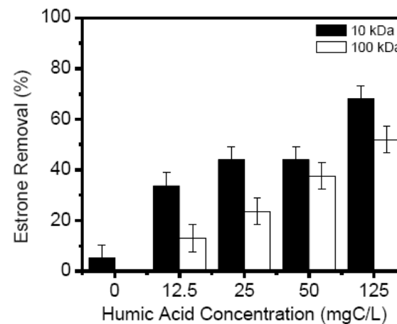
Figure 4: Experimental estrone removal ( R_{\%} ) for 10 and 100 kDa MWCO membranes as a function of HA concentration (1 mM NaHCO 3 , 20 mM NaCl, pH 8, 100 ng/L estrone, HA concentrations of 0, 12.5, 25, 50 and 125 mgC/L)
