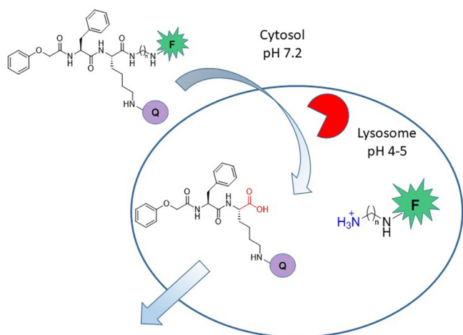
Fig. 6. The fluorophore is attached on the C-terminal side of the cleavable amide bond, whereas the quenching group is attached to the lysine side chain. Upon enzymatic cleavage of the substrate, a fluorescent fragment accumulates in lysosomes due to protonation of the free amine that is produced by the proteolytic process.
