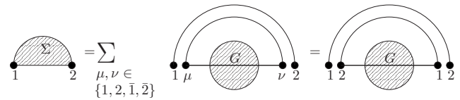
FIG. 4. Example of calculation of \sigma_{12} in Eq. (61). We write the second Dyson-Schwinger equation for \Sigma_{12} . The only nonvanishing propagator is the one between indices 1,2 and 1,2. Taking the trace of both sides of the equation we arrive at \sigma_{12} = \tau_1 g_{21} .
