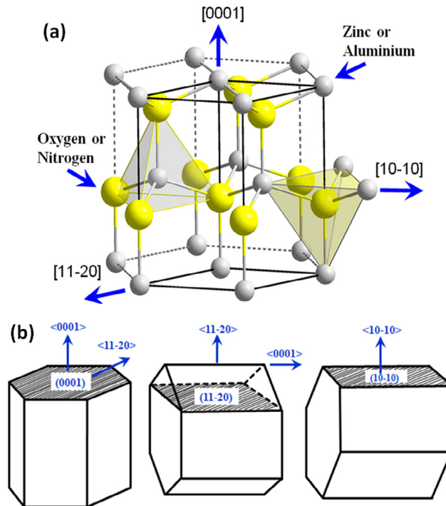
Fig. 8. (a) Illustration of wurtzite type crystal structures of ZnO and AlN including the three key directions; (b) preferred orientations along (0001), (1120) and (1010) planes of ZnO and AlN crystals on film surfaces.
