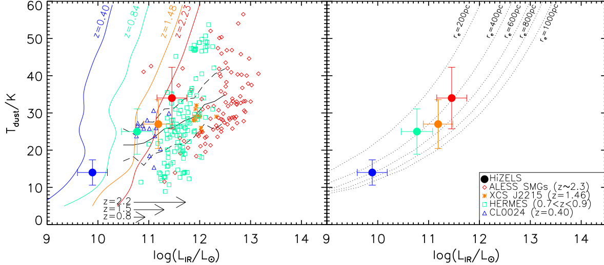
FIG. 3.— Left : Dust temperature, T_{\text{dust}} versus the modified blackbody luminosity, L_{\text{IR}} , for the four extinction-corrected, H \alpha -selected HiZELS samples, using properties measured from the best-fitting SEDs (§ 2.5). HiZELS stacks are plotted with large filled symbols, and use the same colour coding as in Fig. 1. We show the relation for 0.1 < z < 2 IR-luminous star-forming galaxies (black line with \pm 2\sigma scatter) from Symeonidis et al. (2013). Typical selection boundaries are shown with colour-coded lines for each redshift (see text for details). The arrows at the bottom of the plot indicate the expected increase in L_{\text{IR}}^*(z) relative to z = 0.40 , given the evolution in L_{\text{H}\alpha}^*(z) , and the common scaling between L_{\text{H}\alpha} and L_{\text{IR}} proposed in Kennicutt & Evans (2012). This evolution roughly matches that seen in our samples, in the sense that straightforwardly converting L_{\text{H}\alpha}^*(z) to \text{SFR}^*(z) to L_{\text{IR}}^*(z) using the scaling relations of Kennicutt & Evans (2012) places the arrow heads at infrared luminosities that are close to those we measure from the stacks. We also show comparison samples observed in the far-IR at the redshifts of our HiZELS stacks, including a population of ALMA-detected z > 2 submillimetre galaxies (Swinbank et al. 2014), submillimetre-detected starburst galaxies in the z = 1.46 cluster, XCS J2215 (Ma et al. 2015), a population of \langle z \rangle \sim 0.8 far-infrared selected starbursts from Casey et al. (2012), and starburst galaxies in the core of the z = 0.4 cluster CL0024+17 (Johnson et al. 2016). Right : As the left hand plot, but with the comparison samples and the local relation removed. If the dust is well described by a greybody SED, then it ought to obey a modified Stefan-Boltzmann (SB) law, L_{\text{IR}} \propto R^2 T_{\text{dust}}^4 . We show curves of constant size, using the prescription outlined in § 3.4, finding that the dust emission from our H \alpha stacks is well-described as having a constant characteristic size \sim 500 pc, with increasing temperature and luminosity at higher redshifts. We note that this size is \sim 10\times smaller than the median stellar sizes of HiZELS galaxies, which may suggest the dust is bound in clumpier knots and filaments, and does not directly trace the stellar emission.
