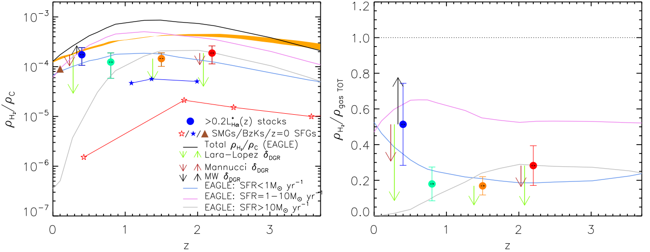
FIG. 4.— Left : The contribution of far-IR stacked > 0.2 L_{H\alpha}^* star-forming galaxies to the total molecular gas ( H_2 ) density of the universe from the EAGLE simulation (Lagos et al. 2015, thick black line). Stacked H \alpha -selected galaxies are shown at z = 0.40, 0.84, 1.47 and 2.23 with filled, coloured points, using the same colour scale as Fig. 1. Gas masses are measured from the dust continuum fits using the Stott et al. (2013) fundamental metallicity relation (FMR) to measure the metallicity from the SFR and \langle M_\star \rangle of each stacked sample, and then using the relation between metallicity and the gas-to-dust ratio ( \delta_{GDR} ) described by Leroy et al. (2011). Coloured arrows to the left of each point show the effect of using the FMR fits of Lara-López et al. (2010) and Mannucci et al. (2010) to derive \delta_{GDR} , or of using a fixed Milky Way \delta_{GDR} = 140 (Draine et al. 2007); we discuss the sensitivity of our results to the choice of FMR relation in detail in Appendix A.2. We do not plot arrows where the change is less than the 1\sigma error on the HiZELS data point. Also shown are the z = 0 data from Kereš et al. (2005), along with higher-redshift BzKs and SMGs from Daddi et al. (2010), Tacconi et al. (2013) and Swinbank et al. (2014), respectively, plus model predictions from Lagos et al. (2015) for the contribution of galaxies with given SFRs. We see that our stacked H \alpha -selected galaxies account for a significant fraction of the gas located in 1-10 M_\odot \text{ yr}^{-1} star-forming galaxies at z = 0.40 and 2.23 . At z = 0.84 and 1.47 , a significant fraction of the gas remains unaccounted for; however our analysis suggests that stacking H \alpha -selected SFGs recovers more of the gas in the universe than is measured by summing individually-detected BzKs/SMGs over the same redshift range. For comparison with EAGLE, we also show the range of H_2 densities from the models of (Popping, Somerville & Trager 2014, orange band). Right : As in the left panel, but normalised by the total gas density. We see that the our stacks all lie below the predicted contribution to \rho_{H_2} from galaxies with SFR = 1-10 M_\odot \text{ yr}^{-1} in EAGLE, indicating that the contribution made by HiZELS H \alpha -selected galaxies to the total gas density is significant, but that our H \alpha cuts have also missed a significant contribution to the gas budget from low-SFR galaxies.
