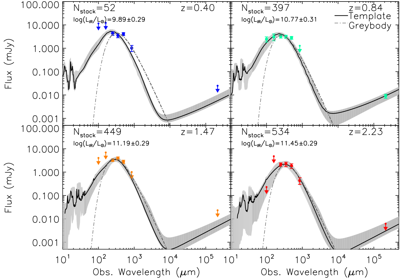
FIG. 1.— Far-infrared/sub-mm spectral energy distributions of stacks comprising all HiZELS star-forming galaxies with L_{H\alpha} \geq 0.2L_{H\alpha}^*(z) , in each of the four redshift slices. Stacked photometry are shown with coloured points; non-detections are represented as 3\sigma upper limits with arrows. We show the best-fitting template SED for each stack, along with the range of templates within \chi^2_{\text{red}} = 1 as a grey band. The best-fitting isothermal grey-body is shown with a dot-dashed line (see § 2.6 for details). The templates implicitly account for the effects of warm dust (which dominates the SED at \lambda_{\text{rest}} \lesssim 100 \mu\text{m} wavelengths); however in order to facilitate comparison with the literature, we take L_{\text{IR}} to be the integral under the isothermal greybody, representing the dominant cold dust component only.
