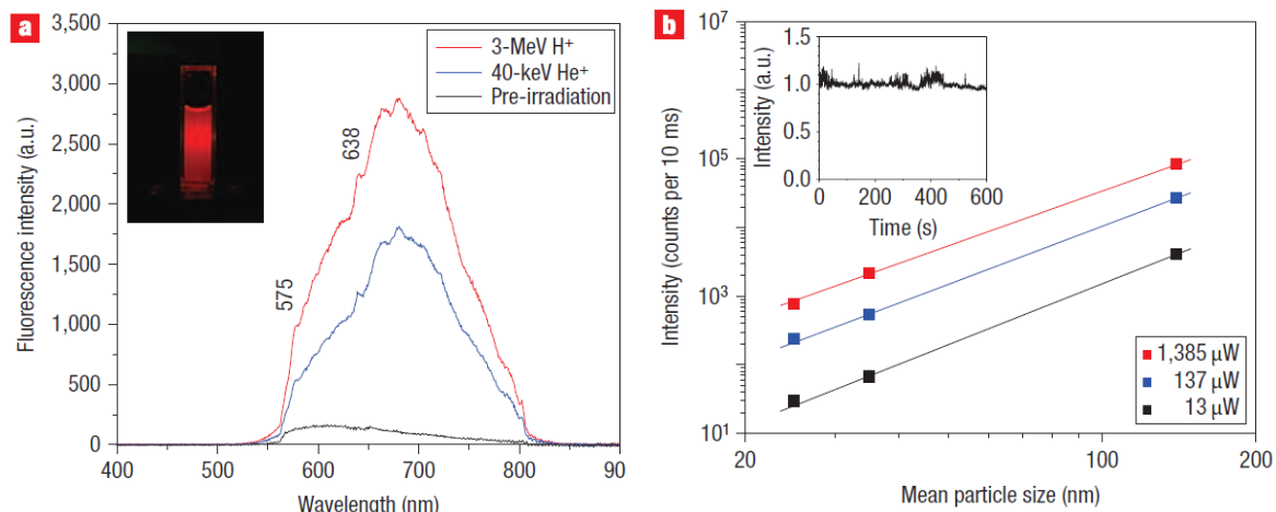
Fig. 6 Characterization of fluorescent nanodiamonds (FNDs). (a) Fluorescence spectra of 35-nm FNDs suspended in water (1 mg ml -1 each), prepared with either 40-keV He + or 3-MeV H + irradiation. Inset: Fluorescence image of a 35-nm FND suspension excited by 532-nm laser light. (b) Fluorescence intensities of FNDs as a function of particle size at three different laser powers. Each data point is the mean of measurements for more than 15 different FNDs. The slopes of the linear fits vary from 2.65 to 2.95 over the power range used in the measurements. Inset: Fluorescence time trace (intensity normalized) of a 25-nm FND. 80
