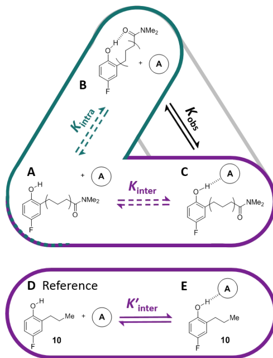
Figure 2. Competition of intramolecular folding A) to B) with intermolecular binding to an external acceptor C). Experimentally non-observable equilibria are indicated with dashed arrows. D) and E) Reference complex used to estimate K_{\text{inter}} .
