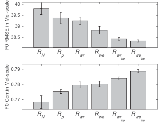
Figure 2: Average objective results on F0 prediction. Each system was trained twice with random initialization, and the models given by the last five training epochs of each trial were used to predict F0. The error bar shows the standard deviation of the ten sets of results for each system.
