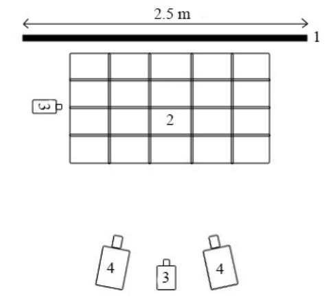
Fig. 2. Arrangement of thermal imagers: 1 - screen 2 - plot for the collection of particles, 3 - video cameras, 4 - thermal imagers.
