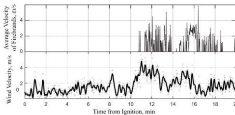
Fig. 7. Wind characteristics and average velocity of firebrands versus time.
