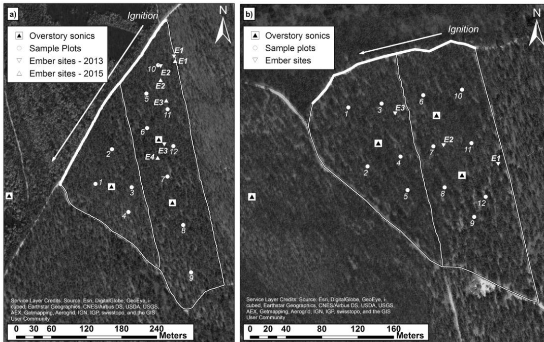
Fig. 1. Location of 4 overstory towers, 12 plots for collection of fuels and 3 plots for collection of firebrands for EX1, EX3 (a) and EX2 (b).
