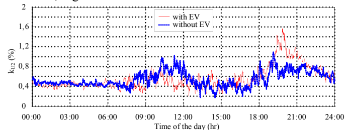
Fig. 1. Impact of a group-connection of EV chargers on negative sequence voltage unbalance, [43].
