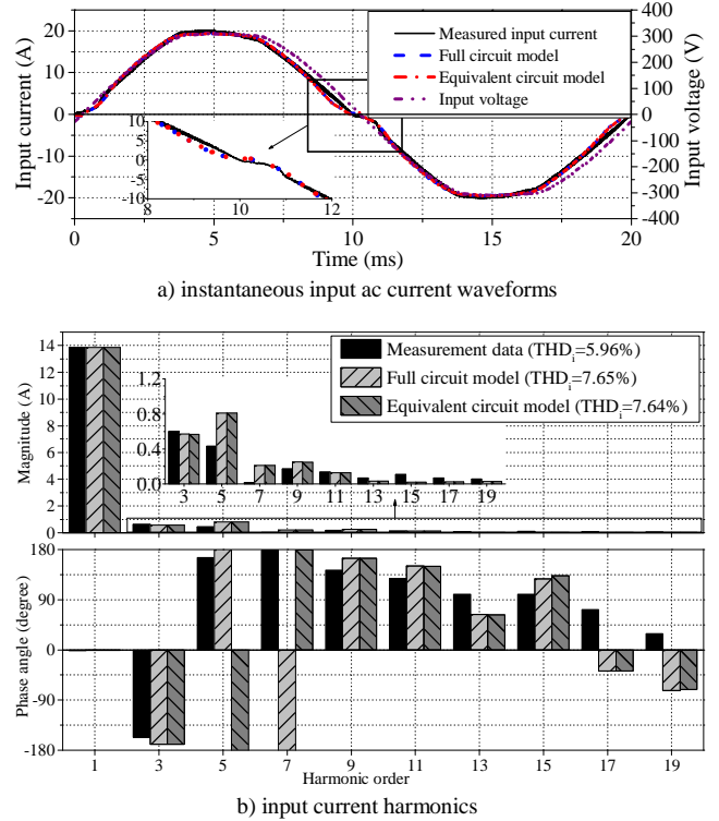
Figure 12. Comparison of measured and simulated input ac currents for 1 pu "flat-top" distorted input ac supply voltage.
