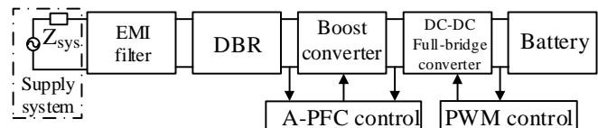
Figure 1. Main components of a single-phase unidirectional EVBC.
