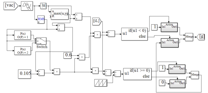
Figure 3. The developed a-PFC control circuit.
