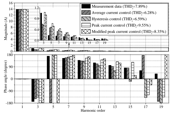
Figure 4. Comparison of input ac current harmonic magnitudes, phase angle and THD values between measurements and considered a-PFC circuits.
