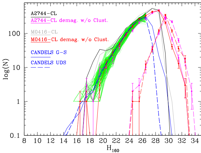
Fig. 7. Demagnified (median magnification, see text for details) H160 number counts in the cluster fields. Magenta and red continuous curves refer to A2744 and M0416 H -detected sources respectively after excluding all objects with photo- z consistent with the redshift of the clusters. Magenta and red dashed lines show the demagnified number counts of additional IR-detected sources (with S/N(H160) > 1 ) in each field. As a comparison, number counts normalized to the FF area from the public CANDELS GOODS-South (Guo et al. 2013) and UDS (Galametz et al. 2013) catalogues are shown as continuous and dashed blue lines, respectively. The green lines are number counts from randomly chosen portions of the CANDELS GOODS-South and UDS field, having the same area as the FF pointings.
