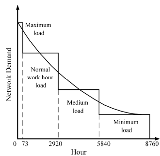
Fig. 1. Load duration curve.
