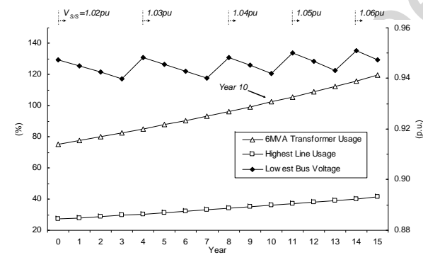
Fig. 3. Yearly analysis of the 69-bus network during peak load (no new generation capacity). Taps at the substation ( V_{S/S} ) are set to maintain voltage profiles within statutory limits.
