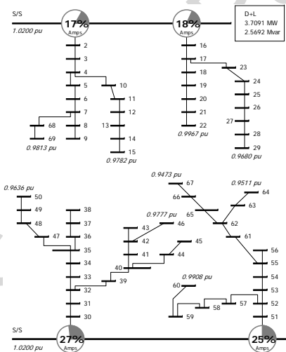
Fig. 2. 69-bus network one-line diagram. Power flow results considering base year and peak load (Table 1).D+L: Total demand and line losses.
