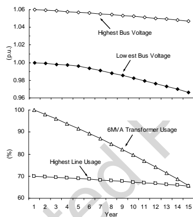
Fig. 4. Yearly analysis of the 69-bus network considering DG Operating Scenario D – Diesel Generator.
