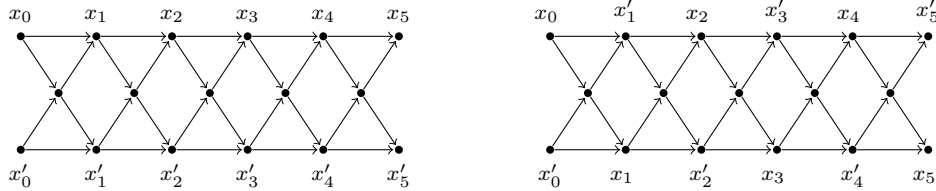
Fig. 8: Example of the construction in Lemma 6 for the view defined in Example 1, that is V = \{C, V\} with C = \{2\} and V = \{1, 2\} . For this example, d = 2 , n = 5 and o = 1 . Remark how the left and right databases agree on V , while there exists a path of length 5 going from x_0 to x_5 in the left database, but no such path in the right one.
