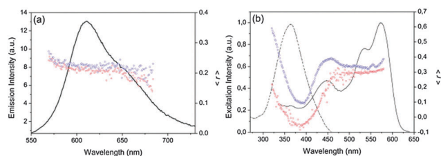
Fig. 6 Steady-state anisotropy of the fluorescence (a) emission ( \lambda_{\text{ex}} = 500\text{ nm} ) and (b) excitation ( \lambda_{\text{em}} = 630\text{ nm} ) of PDI-Sil-d-U(600) (red open squares) and PDI-Sil-d-U(4000) (blue open circles). The emission and excitation spectra (black lines) obtained using non-polarised light are shown for comparison.
