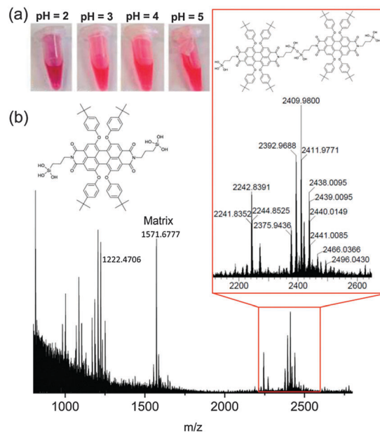
Fig. 2 Acid-catalysed hydrolysis of PDI-Sil under the ureasil reaction conditions. (a) Photographs of a PDI-Sil solution in THF (10 -4 mol dm -3 ) upon ageing at different pH (24 h). (b) MALDI-TOF mass spectrum of the PDI-Sil solution following addition of the catalyst (aq. HCl/EtOH).
