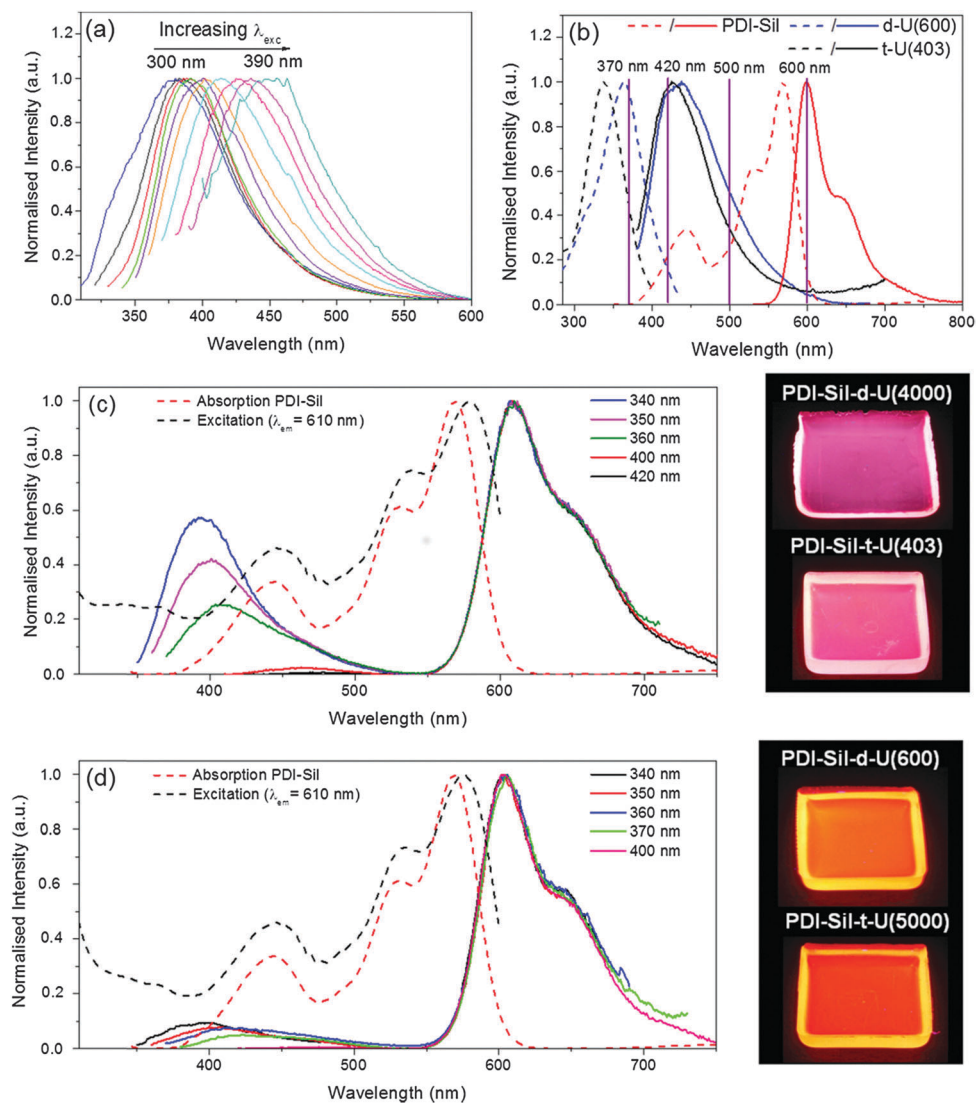
Fig. 4 Steady-state photoluminescence properties of undoped and PDI-Sil -ureasils. (a) PL emission of t-U(403) as a function of the excitation wavelength. (b) PL and excitation spectra for t-U(403) (black, \lambda_{\text{exc}} = 370 nm, \lambda_{\text{em}} = 420 nm), d-U(600) (blue, \lambda_{\text{exc}} = 365 nm, \lambda_{\text{em}} = 420 nm) and UV/Vis absorption and emission spectra for PDI-Sil (red, \lambda_{\text{exc}} = 590 nm in THF ( 1 \times 10^{-6} mol dm ^{-3} )). The purple lines highlight the excitation ( \lambda_{\text{exc}} ) and emission ( \lambda_{\text{em}} ) wavelengths used in the ps-TCSPC experiments. Absorption spectrum of PDI-Sil in THF, PL emission spectra and excitation spectrum ( \lambda_{\text{em}} = 610 nm) of (c) PDI-Sil-t-U(403) and (d) PDI-Sil-t-U(5000) and the corresponding photographs of PDI-Sil -ureasils under UV excitation ( \lambda_{\text{exc}} = 365 nm). Emission spectra are shown as solid lines and excitation and UV/Vis absorption spectra are shown as dashed lines.
