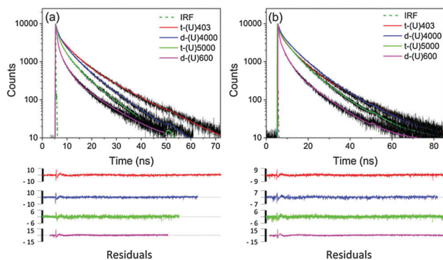
Fig. 5 Emission decay curves (solid black lines) and fits (coloured lines) for undoped ureasils upon excitation at 370 nm and detection at (a) 420 nm and (b) 500 nm. The weighted residuals for each fit and the instrument response function (IRF, dotted line) are also shown.
