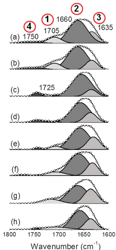
Fig. 3 Gaussian fits to the Amide I region of the FTIR spectrum of (a) d-U(600) , (b) PDI-Sil-d-U(600) , (c) d-U(4000) , (d) PDI-Sil-d-U(4000) , (e) t-U(403) , (f) PDI-Sil-t-U(403) , (g) t-U(5000) , (h) PDI-Sil-t-U(5000) . The circled numbers represent the peaks described in the text.
