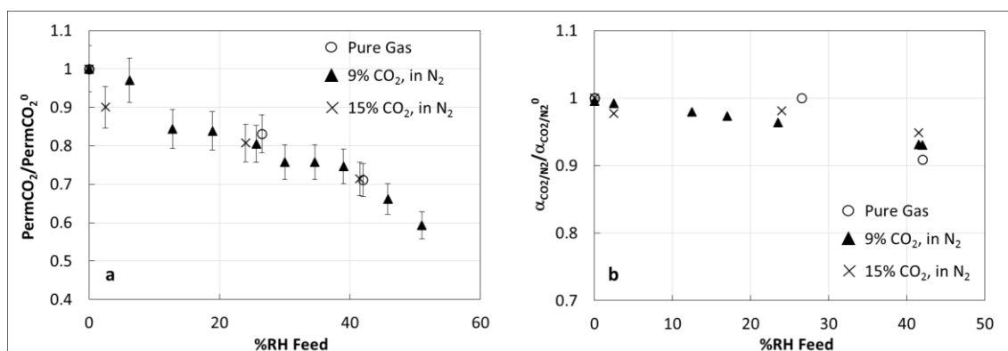
Figure 7: Variation of the CO 2 permeability in humidified CO 2 -N 2 feed versus the feed relative humidity (a) and CO 2 /N 2 selectivity in humidified CO 2 -N 2 feed (b) of PIMI for 3 compositions (Pure gas, 9%CO 2 in N 2 , 15%CO 2 in N 2 ). (P feed =1.3 bar, T cell =35° C. PermGas = permeability in wet conditions; PermGas 0 = initial permeability in dry conditions). (Error calculated by sample repetition)
