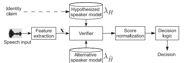
Fig. 2. Diagram of a speaker verification system.
