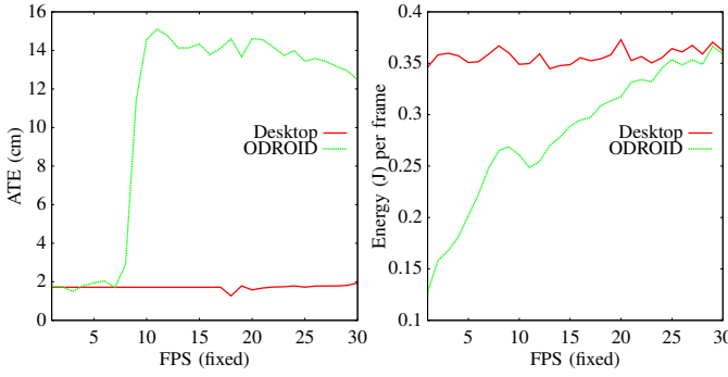
Fig. 4: Varying the input frame-rate in LSD-SLAM under the TUM RGB-D fr2/xyz dataset without using process-every-frame mode. Shows ATE and energy under Desktop and ODROID.
