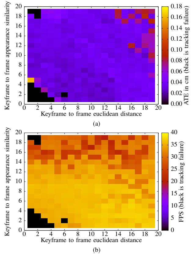
Fig. 3: 2D design space exploration of appearance similarity and distance between frames in LSD-SLAM using TUM RGB-D fr2/desk on Desktop with otherwise default parameters. The heatmap represents: (a) ATE (cm), (b) FPS.
