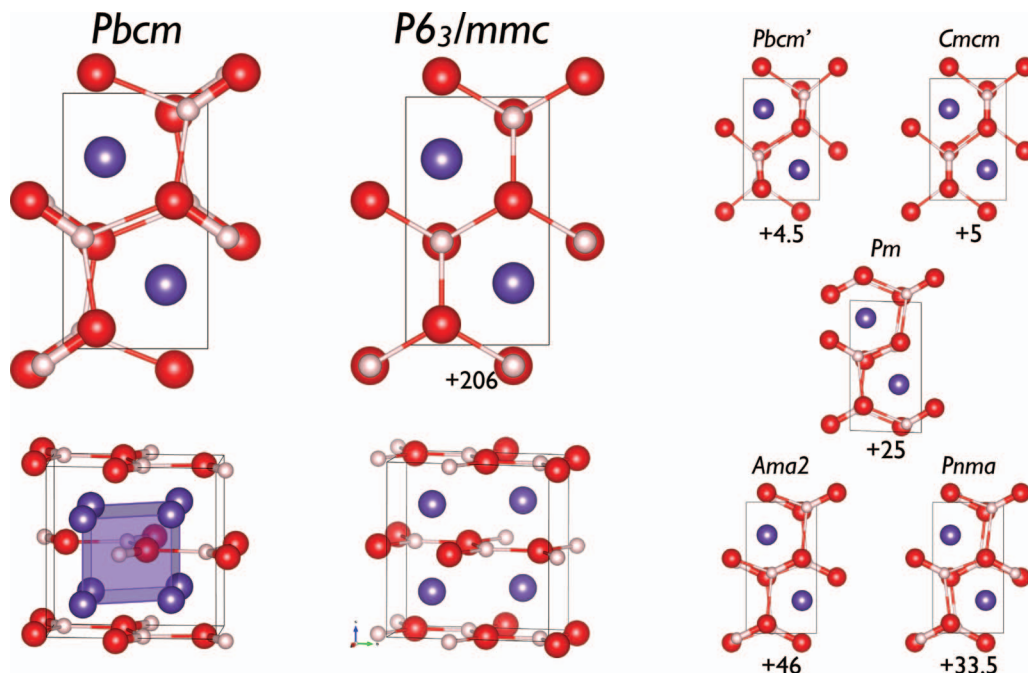
FIG. 8. From left: Pbcm structure of LiOH-IV, top and side view with OH coordination environment; the high-symmetry atomic P6 3 /mmc phase in the same views; and the five other distortions of P6 3 /mmc , top views. Numbers indicate metastability per formula unit at P = 300 GPa with respect to Pbcm -LiOH-IV.
