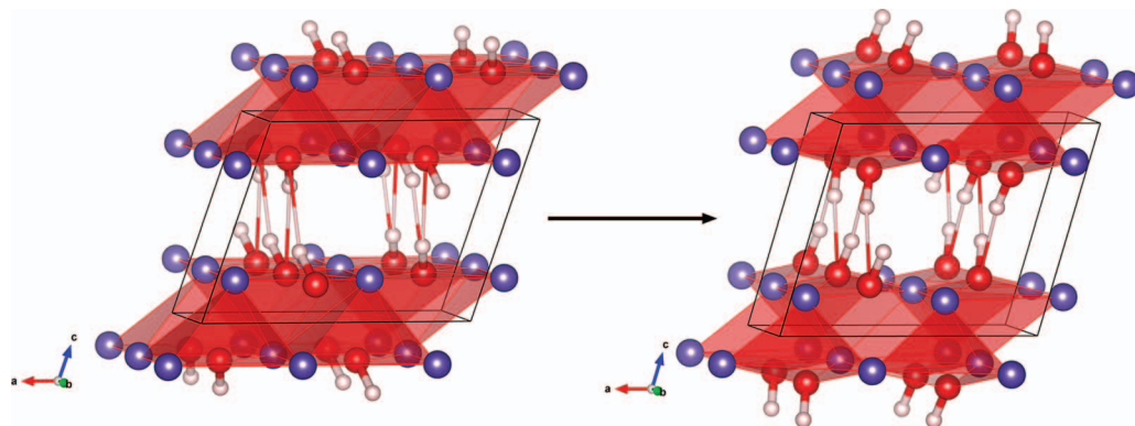
FIG. 7. The P2_1/a structure as proposed at 1.8 GPa (left) and its optimized ground state at 2 GPa (right). Coordination polyhedra of oxygen are indicated in red, and hydrogen bonds by thin lines.
