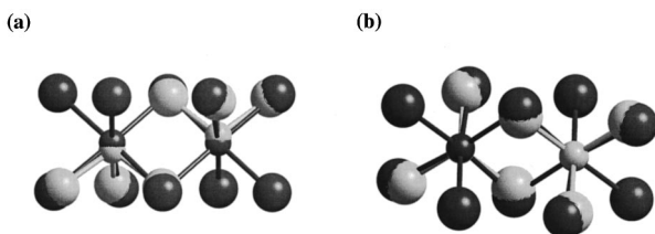
FIG. 5. An illustration of the structural response to compression showing the twisting of SbI 3 molecular units. The lighter and darker spheres correspond to the atomic positions at ambient pressure and 54 kbar, respectively. The small sphere stands for the Sb atom and larger one for the I atom.
