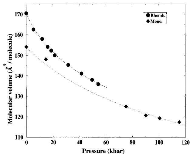
FIG. 9. Molecular volume vs pressure for \text{SbI}_3 illustrating the relatively small volume collapse and the irreversibility of the transition under decompression. The low-pressure phase (rhombohedral) is denoted as the solid circle whereas the high-pressure phase (monoclinic) is shown as the solid diamond. The dashed and dotted lines represent a fit to the Birch-Murnaghan equation of state.
