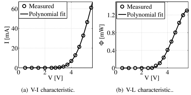
Fig. 10. LED output characteristic.
