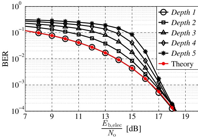
Fig. 3. 16-QAM eU-OFDM performance at different depths as a function of the electrical SNR. The curve “Theory” represents the theoretically-derived performance bound.
