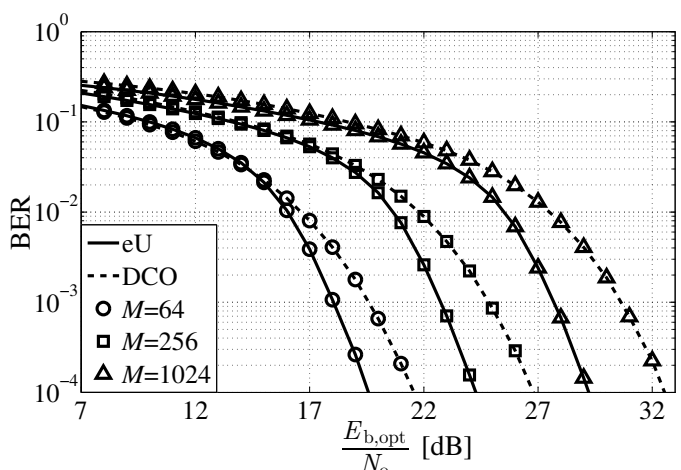
Fig. 8. eU-OFDM performance vs. DCO-OFDM performance for different M -QAM constellation sizes as a function of the optical SNR. Optimum biasing levels for 64-QAM, 256-QAM, and 1024-QAM DCO-OFDM are estimated at respectively 9.5 dB, 11 dB, and 13 dB, as described in (4).
