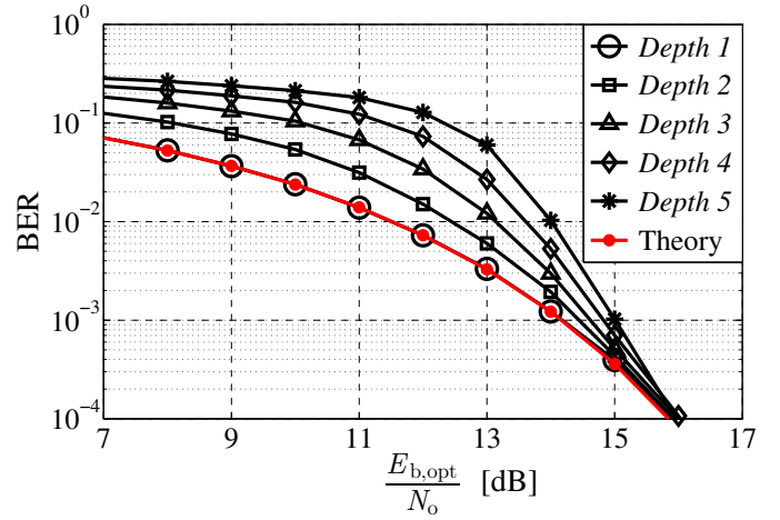
Fig. 4. 16-QAM eU-OFDM performance at different depths as a function of the optical SNR. The curve “Theory” represents the theoretically-derived performance bound.
