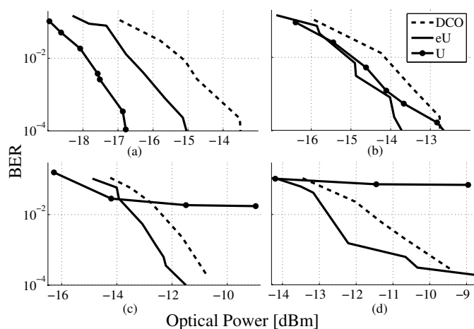
Fig. 13. Performance comparison between eU-OFDM, U-OFDM, and DCO-OFDM for different M -QAM constellation sizes as a function of the optical power measured at the receiver: (a) BPSK (20 Mb/s); (b) 4-QAM (40 Mb/s); (c) 8-QAM (60 Mb/s); (d) 16-QAM (80 Mb/s). All results have been optimized empirically using exhaustive search experiments.
