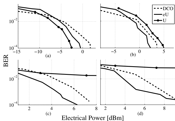
Fig. 12. Performance comparison between eU-OFDM, U-OFDM, and DCO-OFDM for different M -QAM constellation sizes as a function of the electrical power dissipated in the LED: (a) BPSK (20 Mb/s); (b) 4-QAM (40 Mb/s); (c) 8-QAM (60 Mb/s); (d) 16-QAM (80 Mb/s). All results have been optimized empirically using exhaustive search experiments.
