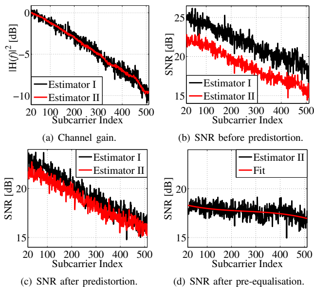
Fig. 11. Communication channel characteristics estimated for an OFDM signal centred at around 3.5 V with a peak-to-peak voltage swing of about 1 V. Subcarriers with indices [0; 20] have not been used for communication due to significant DC-wandering effects at the transmitter, caused by AC-coupling in the bias-T.
