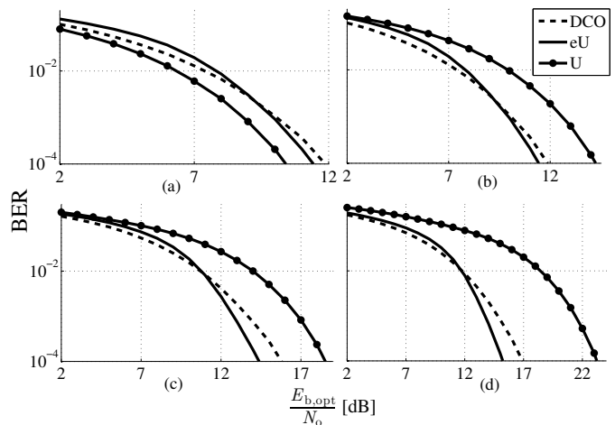
Fig. 7. Performance comparison between eU-OFDM, U-OFDM, and DCO-OFDM for different M -QAM constellation sizes as a function of the optical SNR: (a) BPSK; (b) 4-QAM; (c) 8-QAM; (d) 16-QAM. Optimum biasing levels for BPSK, 4-QAM, 8-QAM, and 16-QAM DCO-OFDM are estimated through Monte Carlo simulations at respectively 6 dB, 6 dB, 7 dB, and 7.5 dB, as described in (4).
