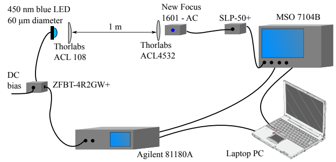
Fig. 9. Experimental set-up.
