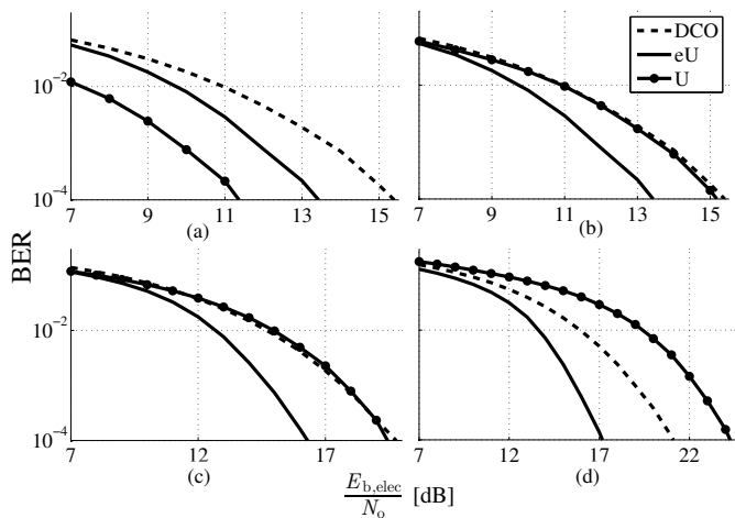
Fig. 5. Performance comparison between eU-OFDM, U-OFDM, and DCO-OFDM for different M -QAM constellation sizes as a function of the electrical SNR: (a) BPSK; (b) 4-QAM; (c) 8-QAM; (d) 16-QAM. Optimum biasing levels for BPSK, 4-QAM, 8-QAM, and 16-QAM DCO-OFDM are estimated through Monte Carlo simulations at respectively 6 dB, 6 dB, 7 dB, and 7.5 dB, as described in (4).
