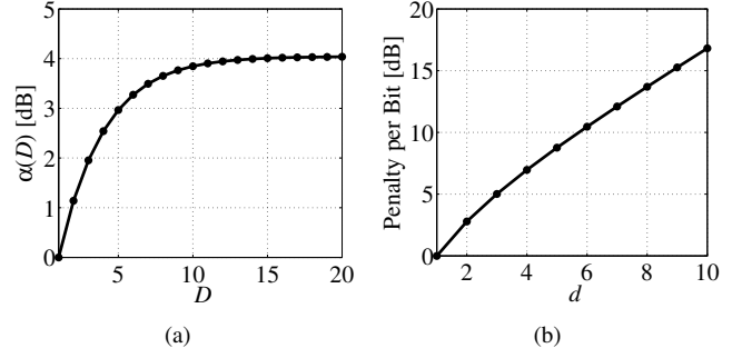
Fig. 2. Energy penalty with increasing modulation depth: a) average penalty per bit as a function of the maximum modulation depth; b) Penalty per additional bit at a specific depth.
