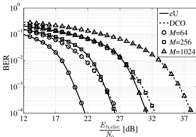
Fig. 6. eU-OFDM performance vs. DCO-OFDM performance for different M -QAM constellation sizes as a function of the electrical SNR. Optimum biasing levels for 64-QAM, 256-QAM, and 1024-QAM DCO-OFDM are estimated at respectively 9.5 dB, 11 dB, and 13 dB, as described in (4).
