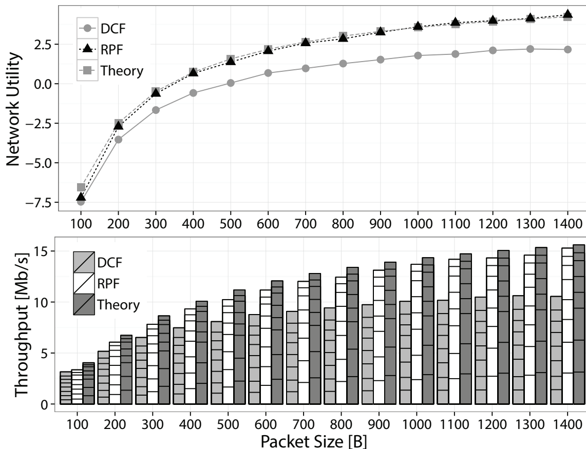
Figure 6: WLAN with 8 backlogged stations transmitting to the AP using UDP. Stations use the OFDM PHY layer (802.11a) and fully heterogeneous bit rates. Network utility (top) and individual/total throughput (below) with standard DCF configuration and the proposed proportional-fair (RPF) allocation scheme as the packet size is varied. Experimental data vs. theoretical optimum prediction.
