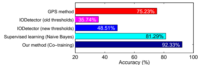
Figure 19. Accuracy comparison of co-training implementation on phone with alternative IO detection approaches.
