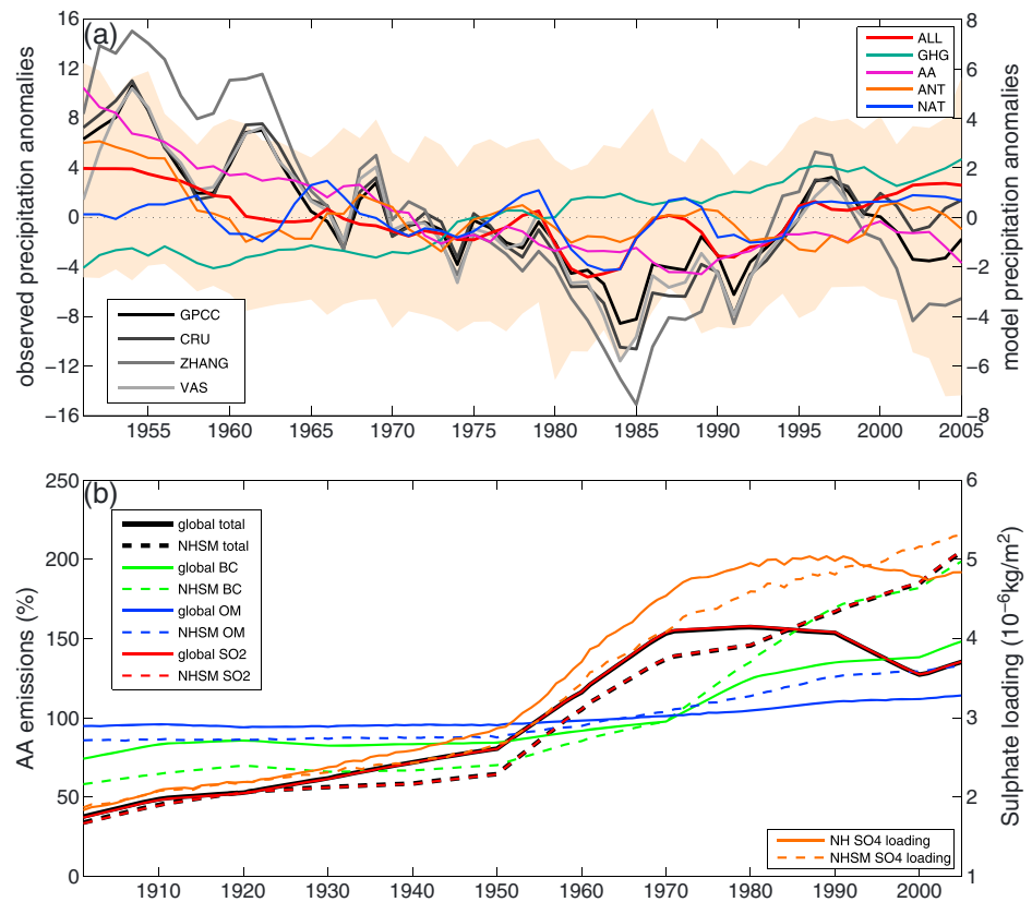
Figure 1. (a) May–September NHSM precipitation anomalies (mm/month) for 1951–2005 for observational data sets, CRU, GPCCC, Zhang, and VasClimO (VasClimO is 1951–2000). Multimodel mean anomalies (different scale to observations) are for all external forcings (ALL), greenhouse gas (GHG), anthropogenic aerosol (AA), natural (NAT), and anthropogenic (ANT) forcing. Anomalies are with respect to 1951–2005 and smoothed with a 5 year running mean. Orange shading shows the ALL ensemble 5%–95% range (same scale as observations). Models are masked to the GPCCC data set. (b) Global and NHSM annual anthropogenic aerosol emissions (% of 1901–2005 mean emissions). NHSM emissions are for 0°–40°N. Total is BC + OM + SO 2 , BC is black carbon, OM is organic matter, and SO 2 is sulfur dioxide. The annual sulfate loadings for the NH and NHSM region are also shown. Aerosol emissions are the CMIP5 emissions based on Lamarque et al. [2010], and sulfate loading is the mean of 11 climate models.
