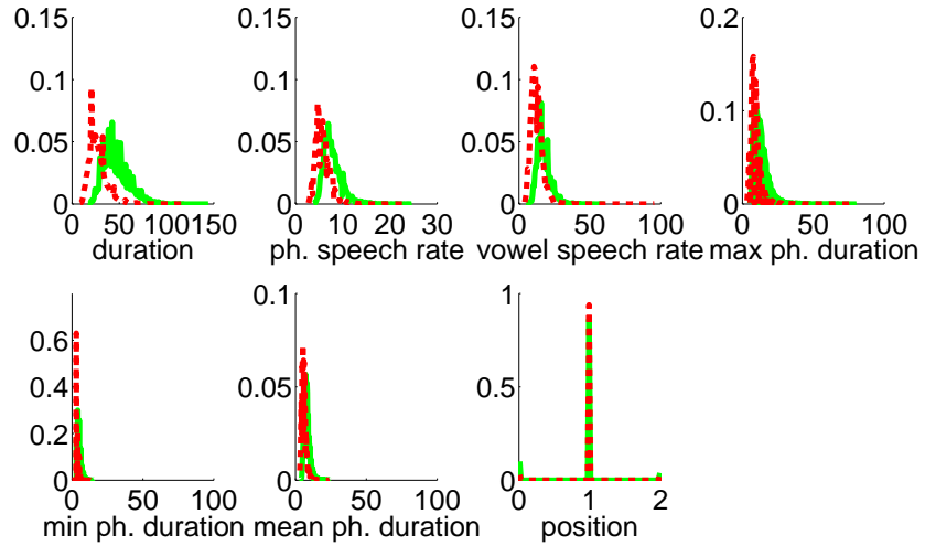
Figure 15: Distributions of the duration-based features and the position feature for Spanish data on the whole development set. The solid green (light grey) curve represents hits and the dashed red (dark) curve represents FAs.
