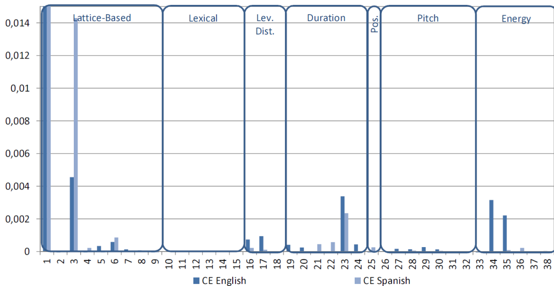
Figure 21: Cross entropy increase with LLR in the leave-one-out experiment for English and Spanish data on the verification set. “Lev. Dist.” refers to the Levenshtein distance-based features. “Pos.” stands for the Position feature.
