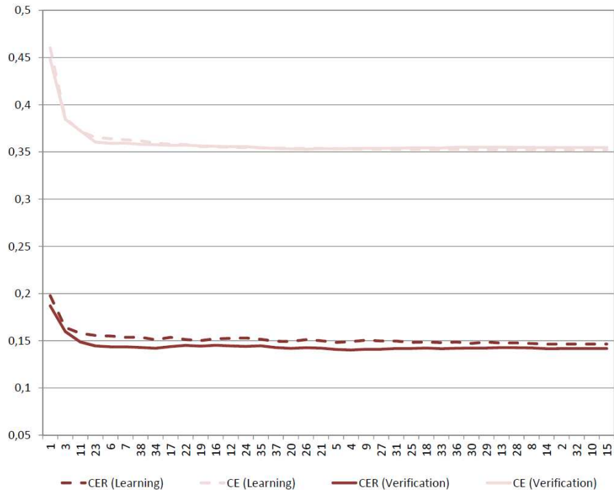
Figure 25: CE and CER results with LLR-based incremental feature selection for English data on learning and verification sets.
