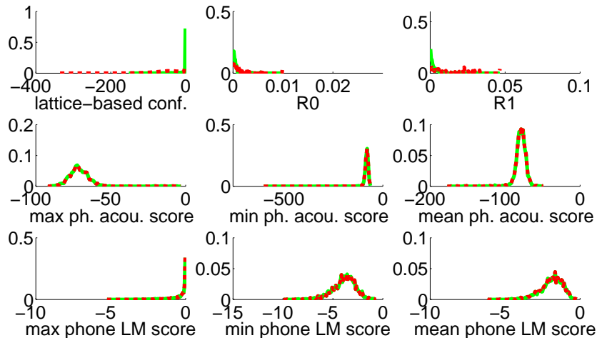
Figure 6: Distributions of the lattice-based features for English data on the whole development set. The solid green (light grey) curve represents hits and the dashed red (dark) curve represents FAs. ‘ph.’ denotes phone, ‘acou.’ denotes acoustic and ‘conf.’ denotes confidence.
