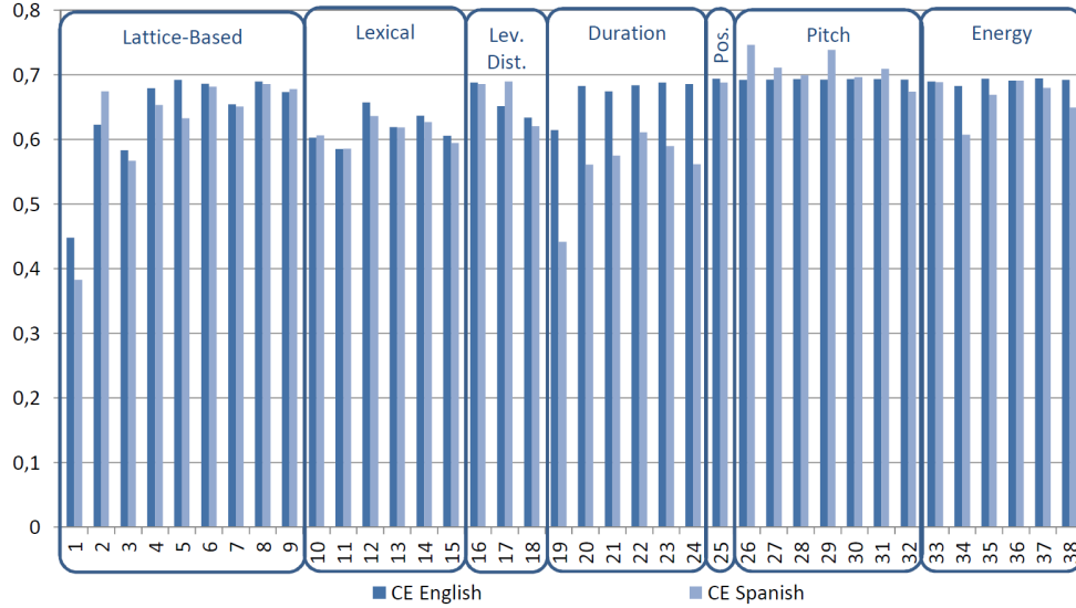
Figure 19: CE obtained for each individual feature for English and Spanish data on the verification set. “ Lev. Dist. ” refers to the Levenshtein distance-based features. “ Pos. ” stands for the Position feature.
