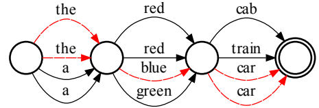
Figure 2: System A: the red cab ; System B: the red train ; System C: a blue car ; System D: a green car ; Reference: the blue car .
