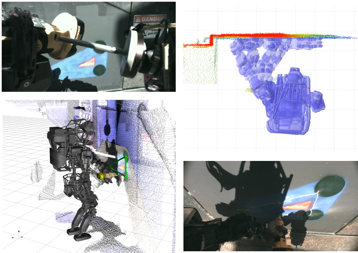
Figure 16: Top left: head camera view of poker used to press drill's power button. Top right: visualization of the nominal plan to reach all drill target points in the triangle. Bottom right: head camera view provides situational awareness to operator as robot executes drilling plan. Bottom left: Robot avatar and RGB point cloud visualization with affordance models of the drill and triangle target.
