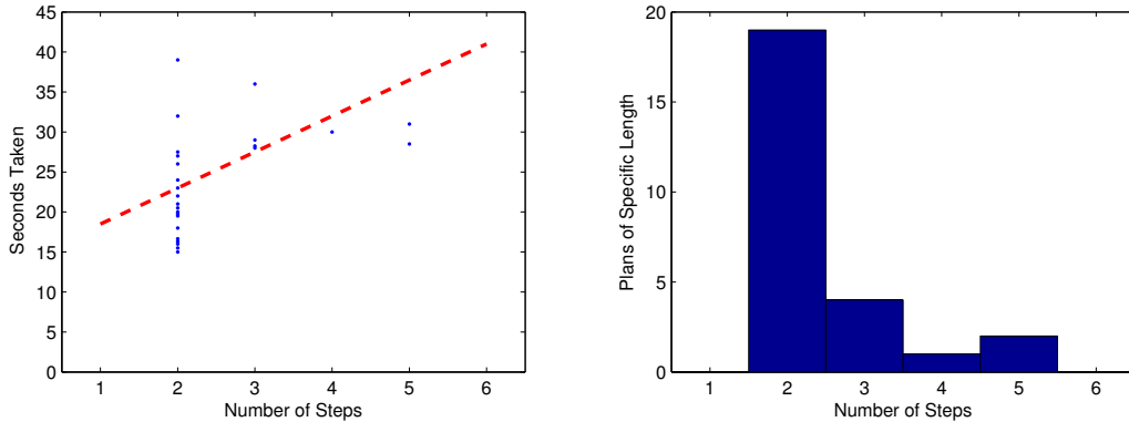
Figure 19: Analysis of Planning for the Walking Task. Left: Time taken to plan (blue dots) and execute (red dashed line) each footstep plan, for different plan sizes. Each blue dot represents the time taken for the operator to place a new set of steps on a terrain map. Right: Distribution of footsteps per walking plan. Typically we limited the robot to just two steps per plan due to state estimate drift.
